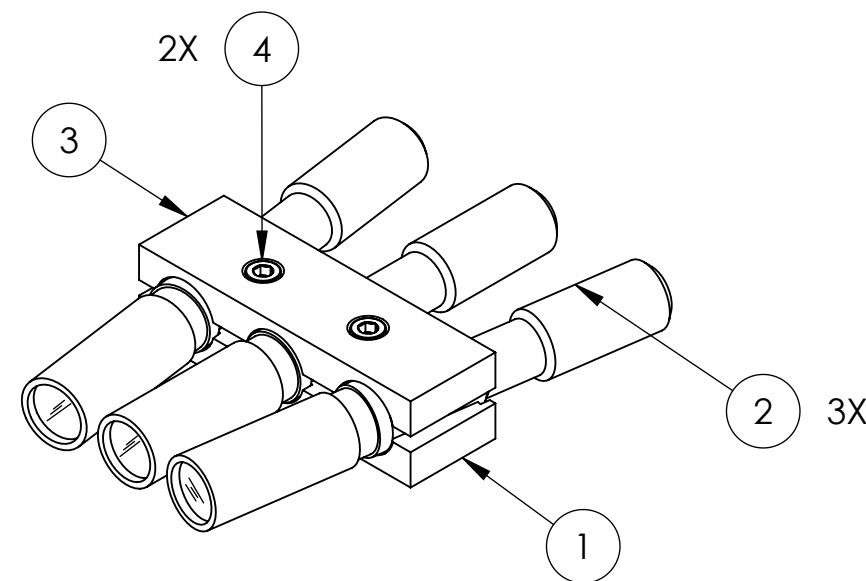
ISO VIEW
