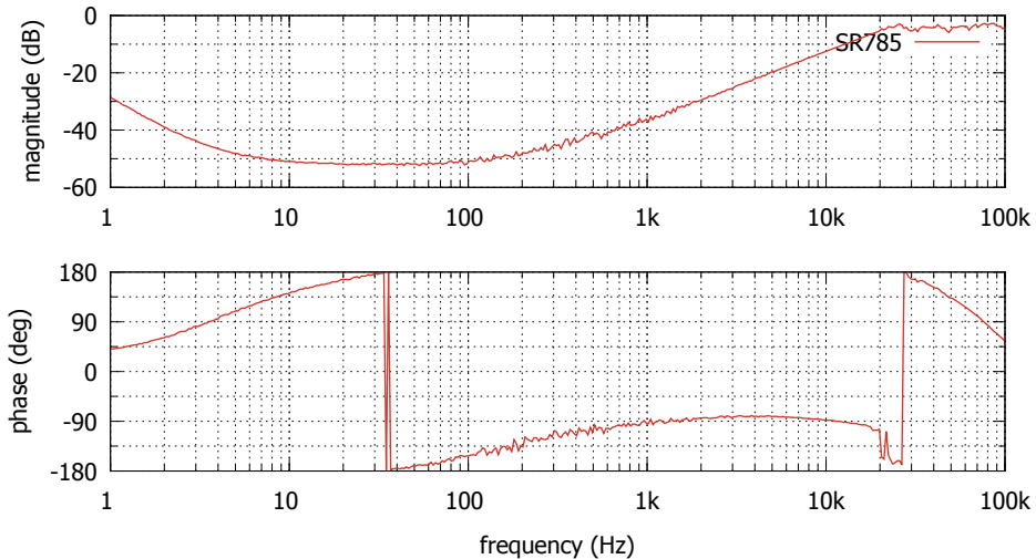
Transfer function ISS second loop injection point photo diode
