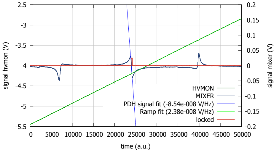
Error signal of PMC
