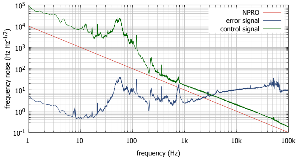
PMC locking frequency noise with FSS
