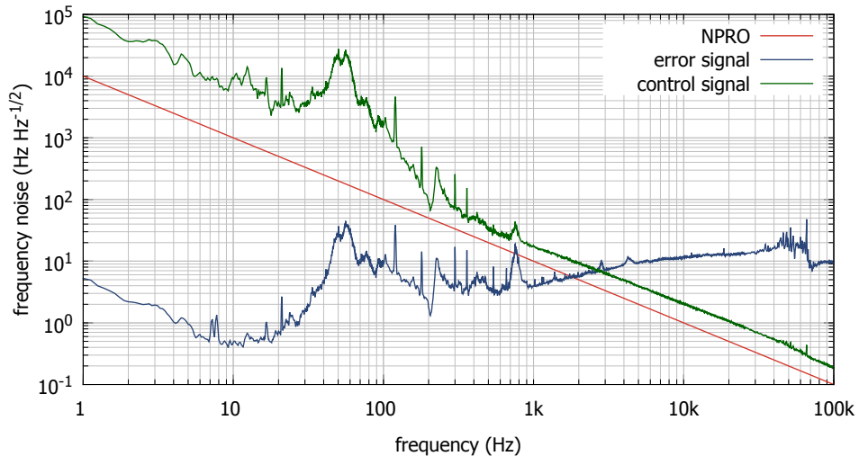
PMC locking frequency noise without FSS
