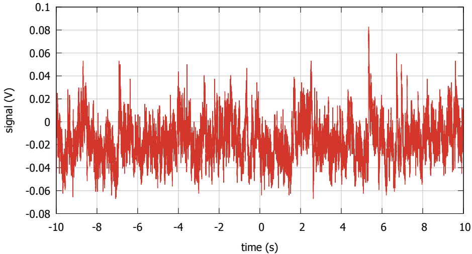
Time series of pockels cell actuator of FSS
