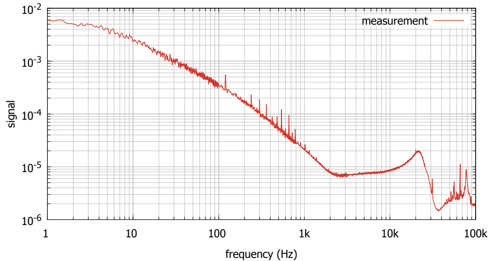
Spectrum of pockels cell actuator of FSS
