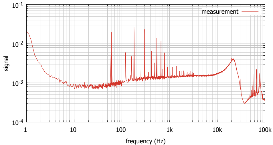
Spectrum of FAST Actuator of FSS
