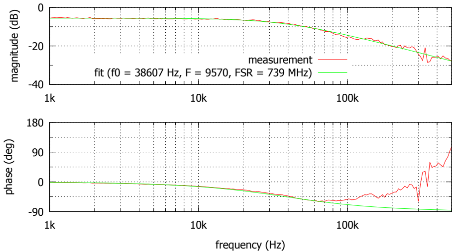
Power modulation transfer function from upstream to downstream of the reference cavity
