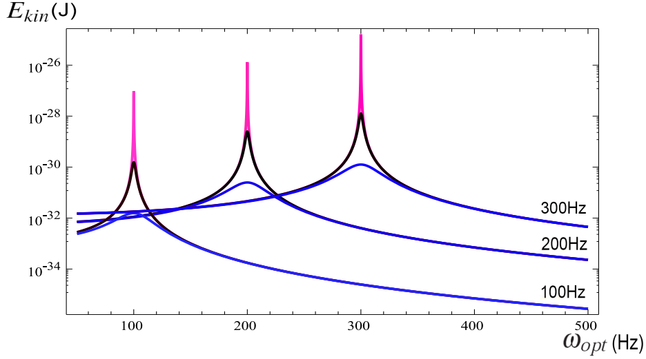
Figure 6. The steady state kinetic energy in a double-spring gravitational interferometer as a function of optical spring frequency due to a monochromatic gravitational wave with h \sim 10^{23} by a LIGO type interferometer. When the gravitational waves have frequency 100Hz, 200Hz and 300Hz, how the optical bar detector with different optical spring frequency (that is, different detuning) responds to them. The red, black and blue lines represent the case when total optical damping \Gamma^{phonon} of the two optical spring is 0.4, 40 and 400Hz respectively. Vertical axis: Energy absorbed, horizontal axis: effective optical spring frequency.
