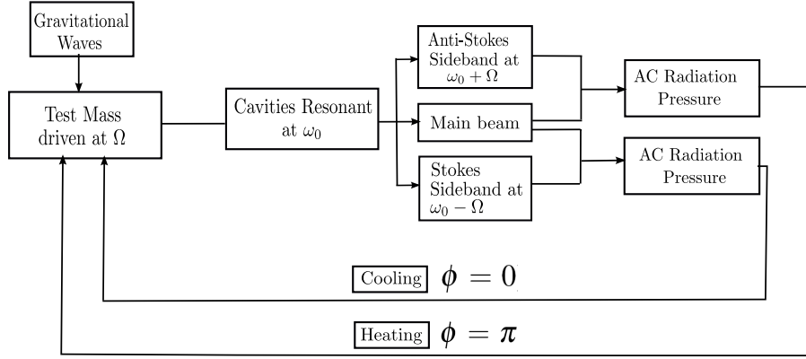
Figure 5. feedback flow chart of cooling and heating effect
