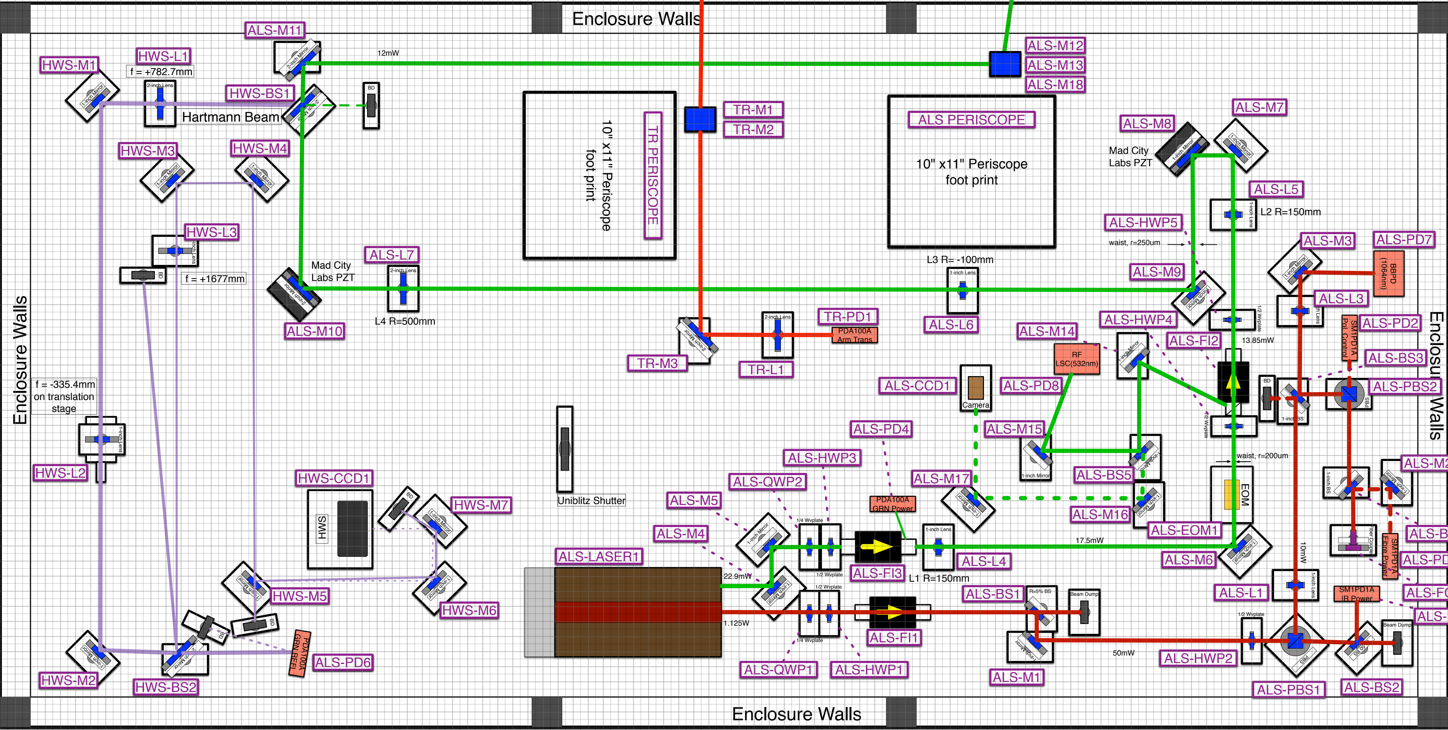
4ft x 8ft optical table, scale = 1:1
