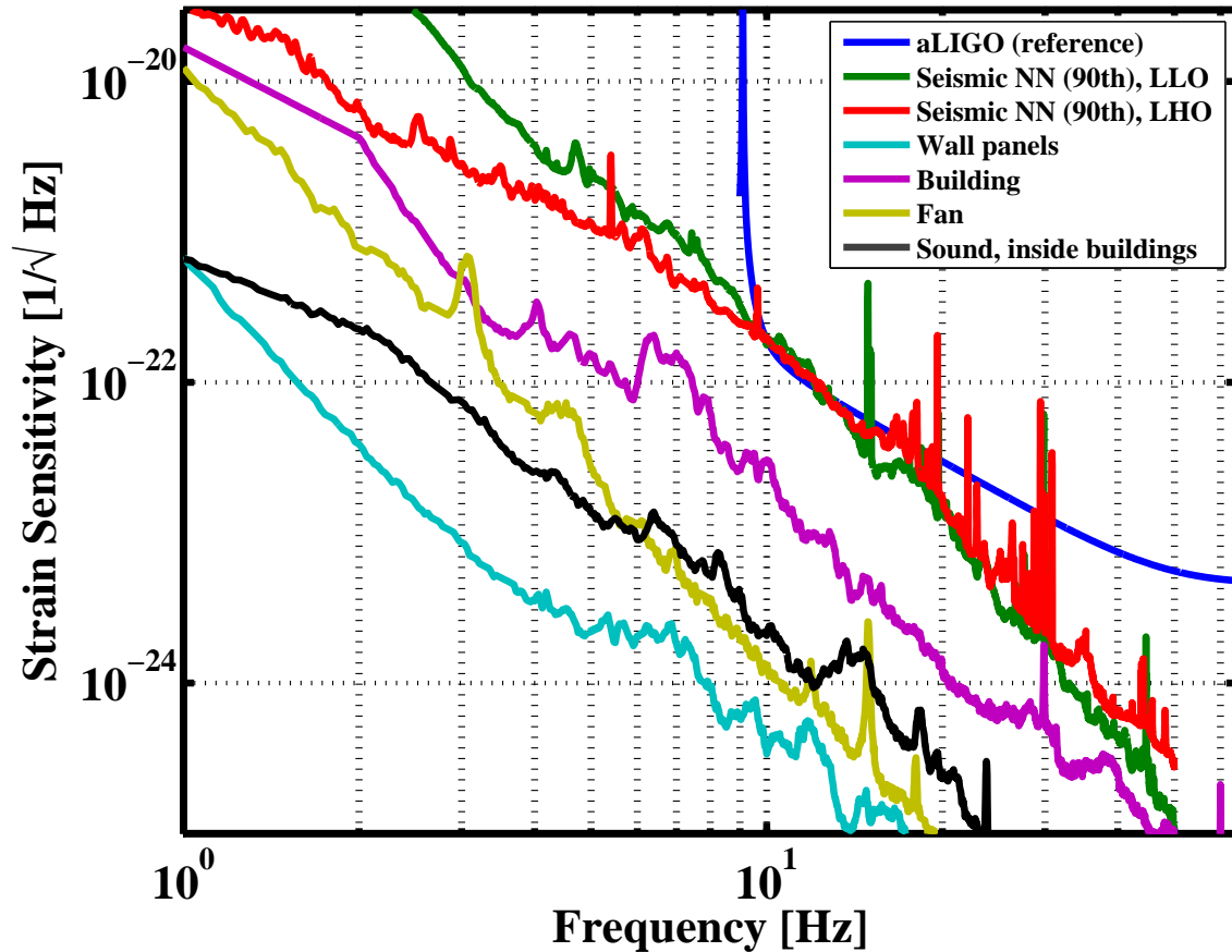
Figure 24: Newtonian noise estimates for the LIGO sites [86]
