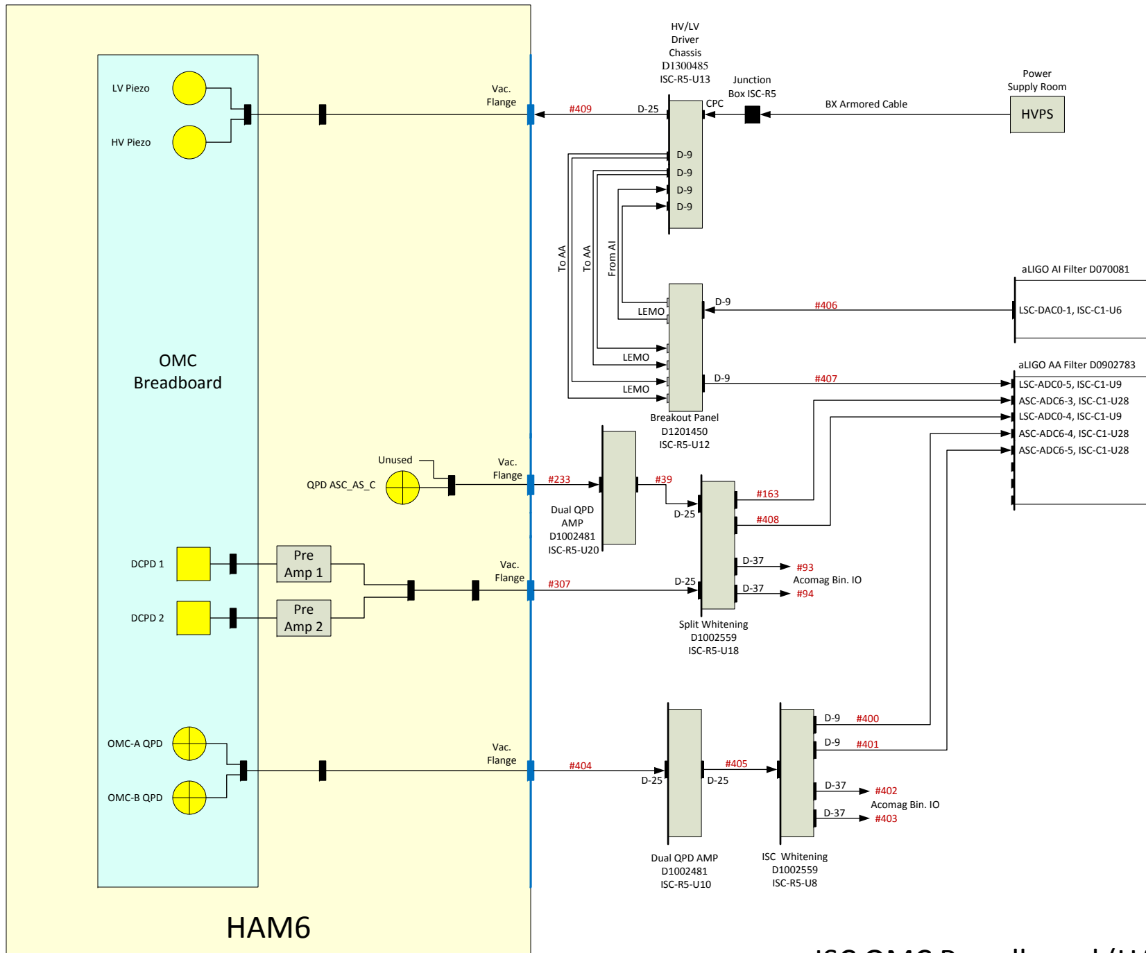
ISC OMC Breadboard (HAM6)
