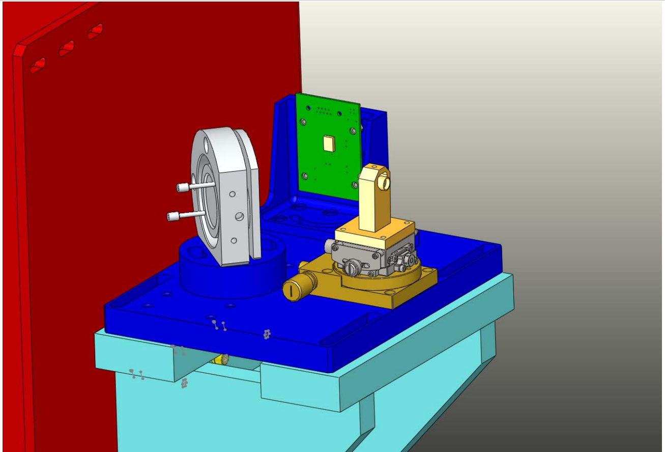
Figure 3: Entire enclosure removed.
