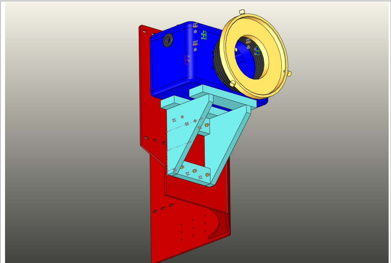
Figure 2: Beam Splitter Transceiver Assembly seen from below
