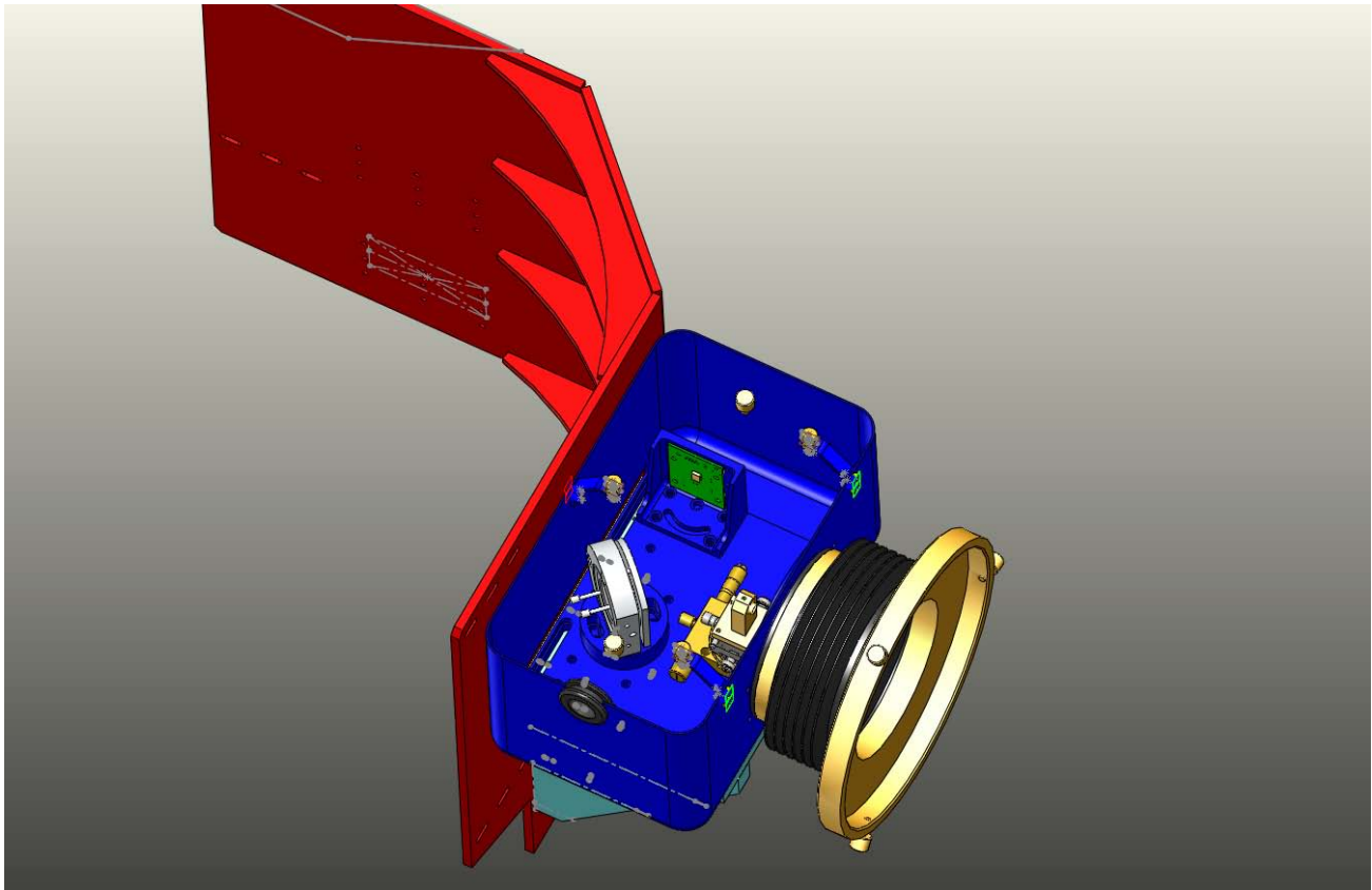
Figure 1: Beam Splitter Transceiver Assembly. Shown with cover removed.
