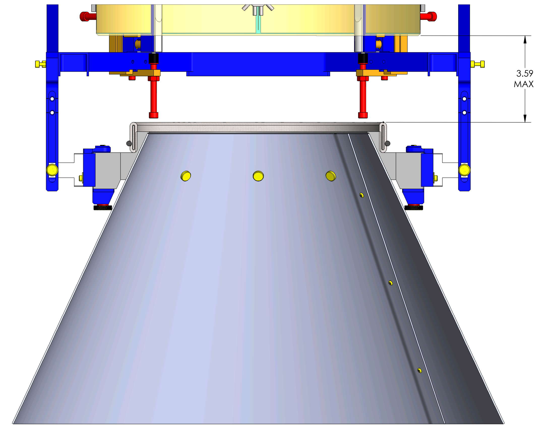
FC SPRAY GUARD, TCP RETRACTED
