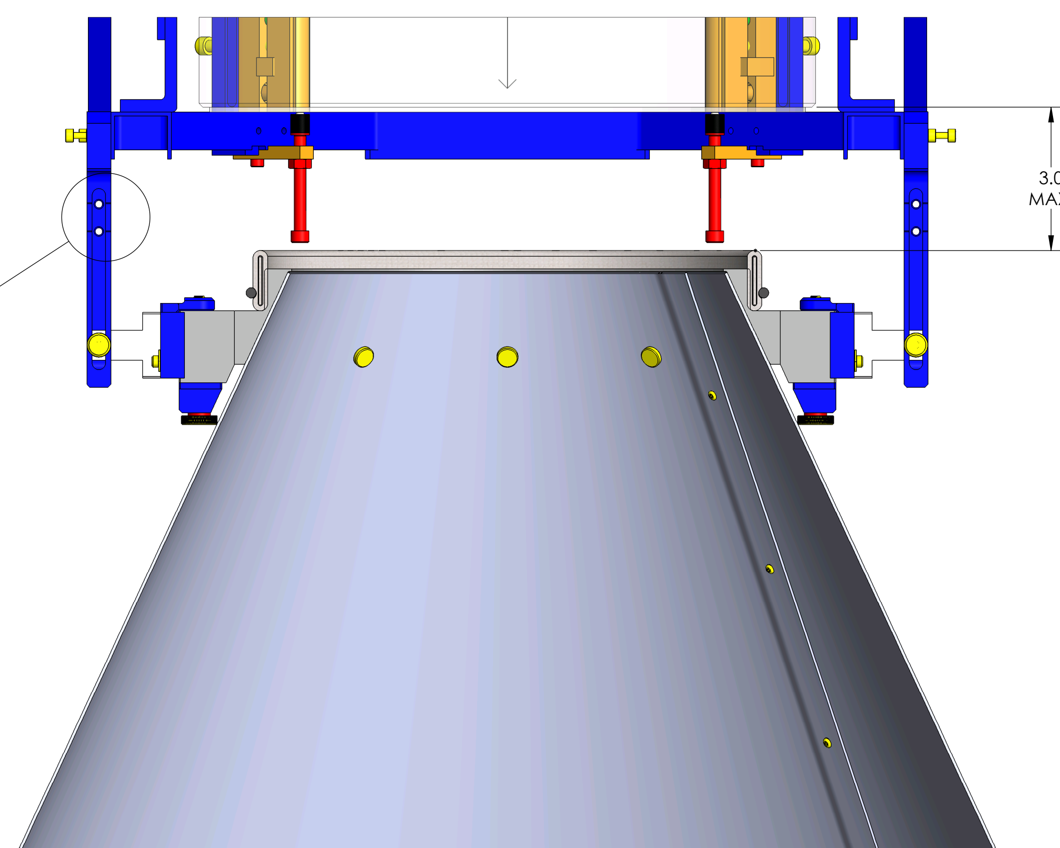
FC SPRAY GUARD, ETM / ITM RETRACTED
