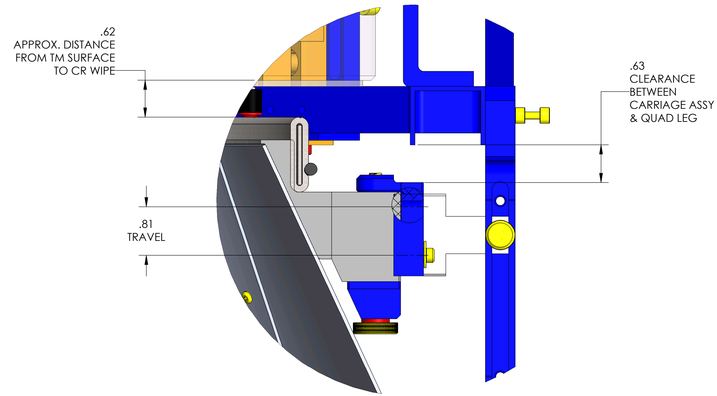
DETAIL B SCALE 1:1
