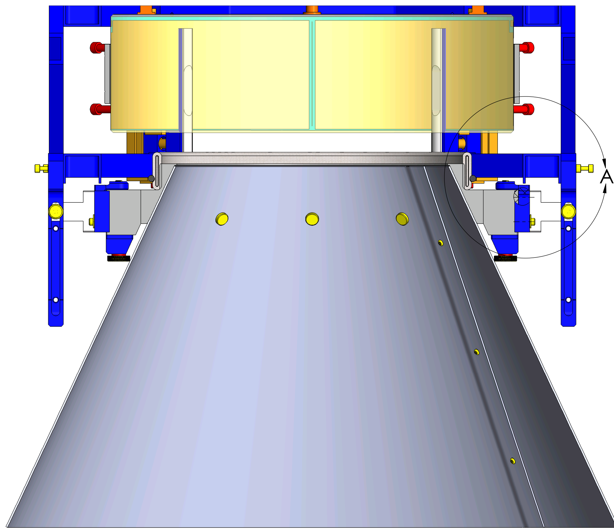
FC SPRAY GUARD, TCP IN-SERVICE
