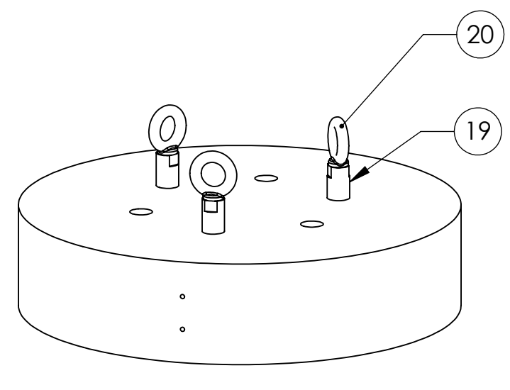
LEG ELEMENT LIFTING HARDWARE
