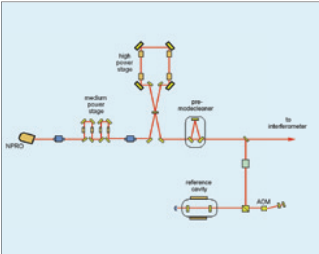
a) Prestabilized laser will be upgraded to 180W
