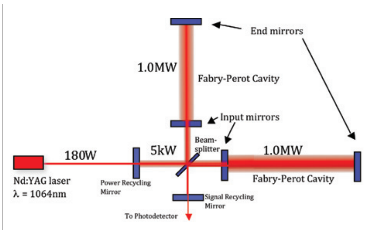
Figure 1.3 Schematic optical design of Advanced LIGO detectors:
