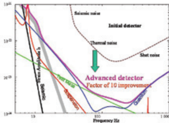
Figure 1.4 Initial LIGO has been a great success, and has shown that it is feasible to reach the sensitivity required.
