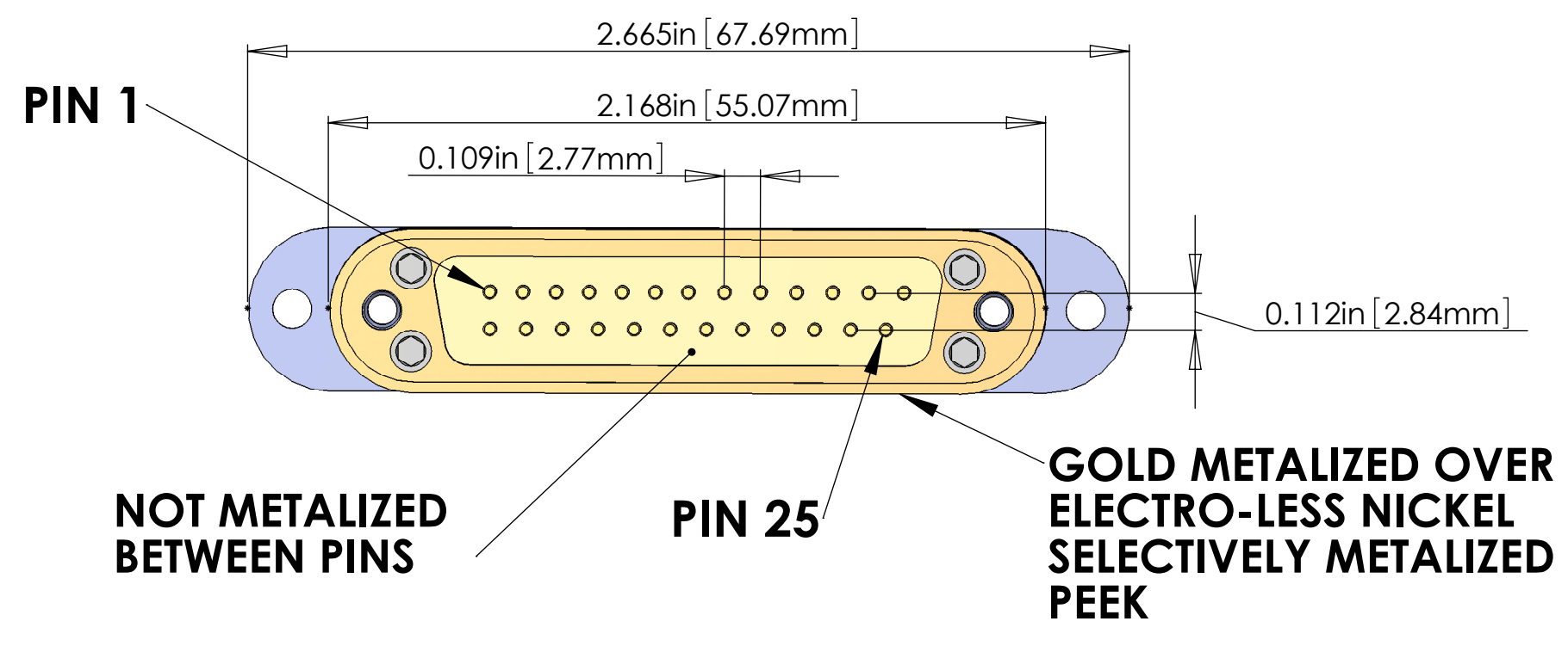
25 PIN D CONNECTOR MALE J1
