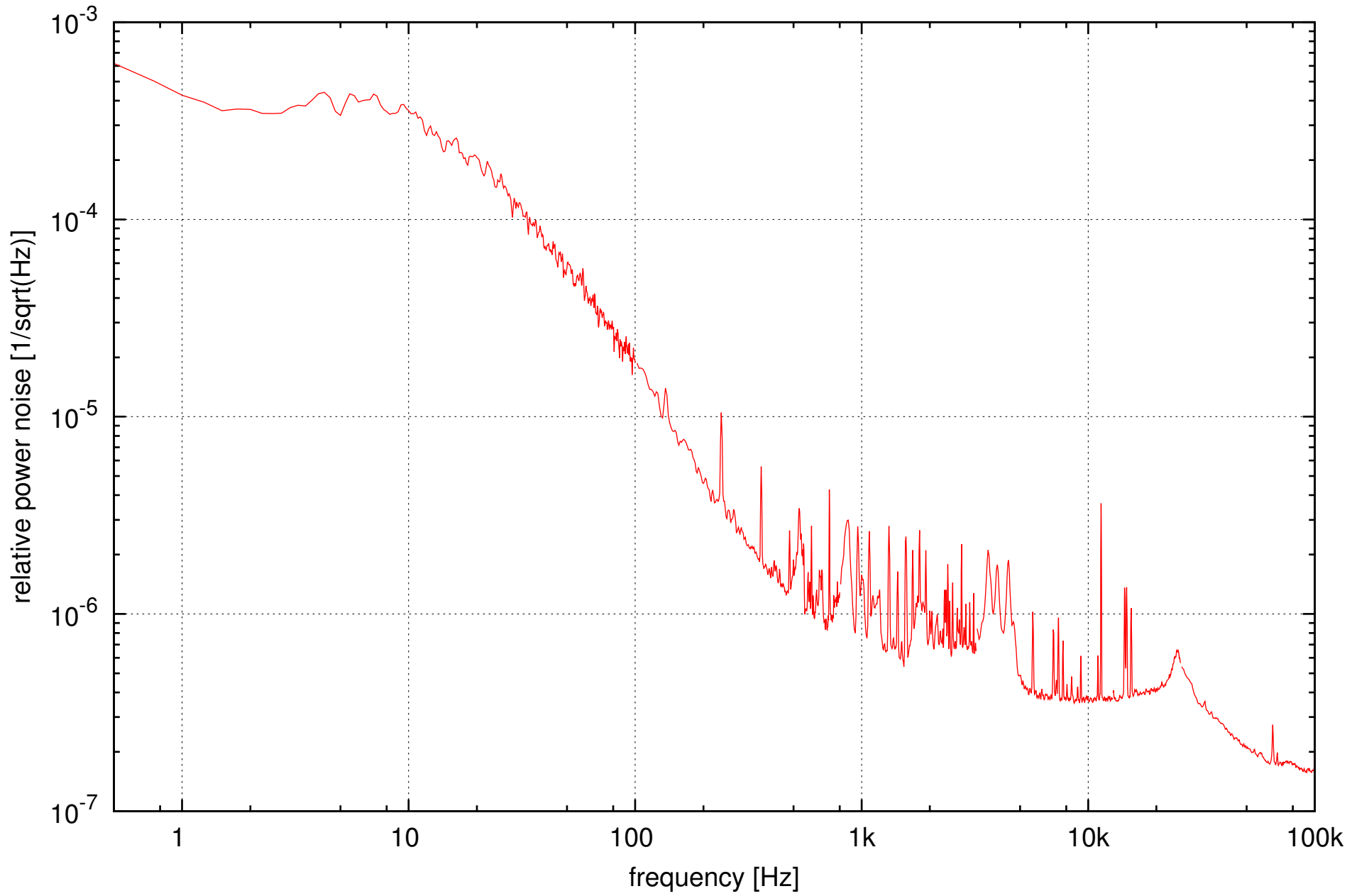
200W laser relative power noise
