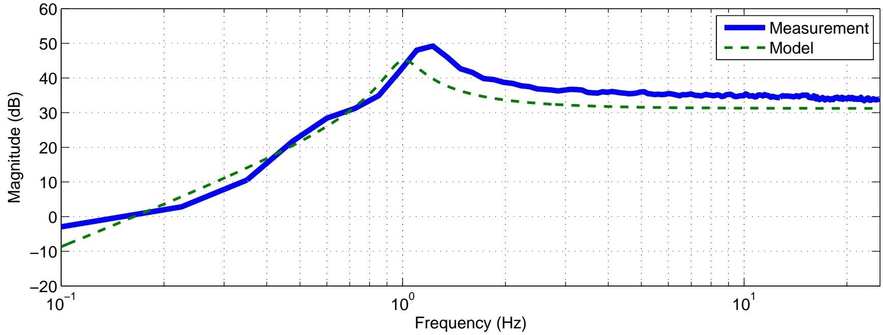
Huddle Test Transfer Function GS-13 SN LV690 / STS SN 109826
