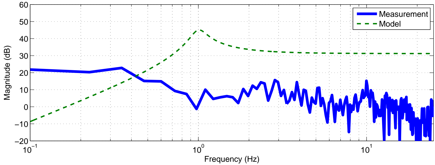
Huddle Test Transfer Function GS-13 SN LH786 / STS SN 109826
