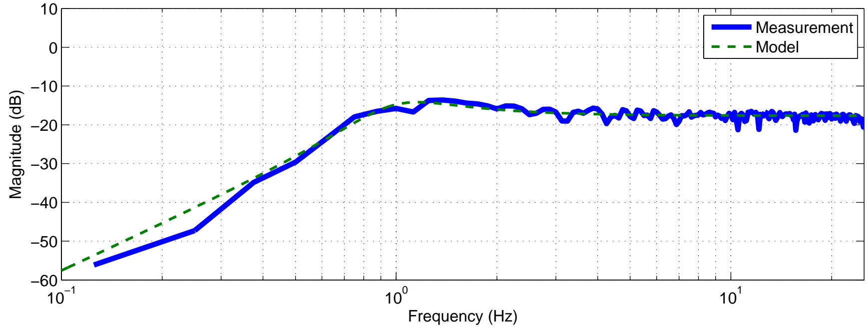
Huddle Test Transfer Function GS-13 SN LH801 / STS SN 109826
