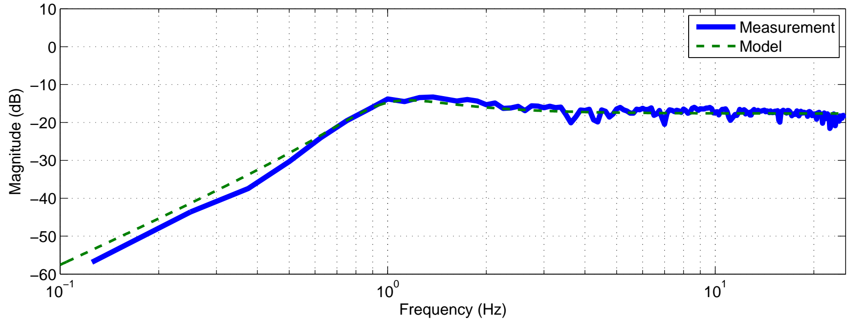
Huddle Test Transfer Function GS-13 SN LH780 / STS SN 109826
