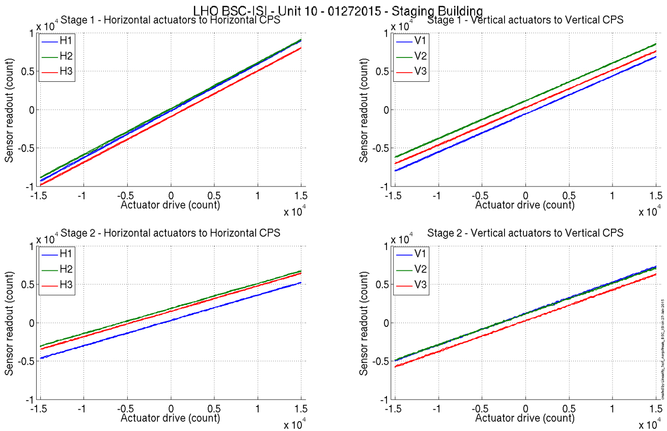
Figure 5 - Linearity Test
