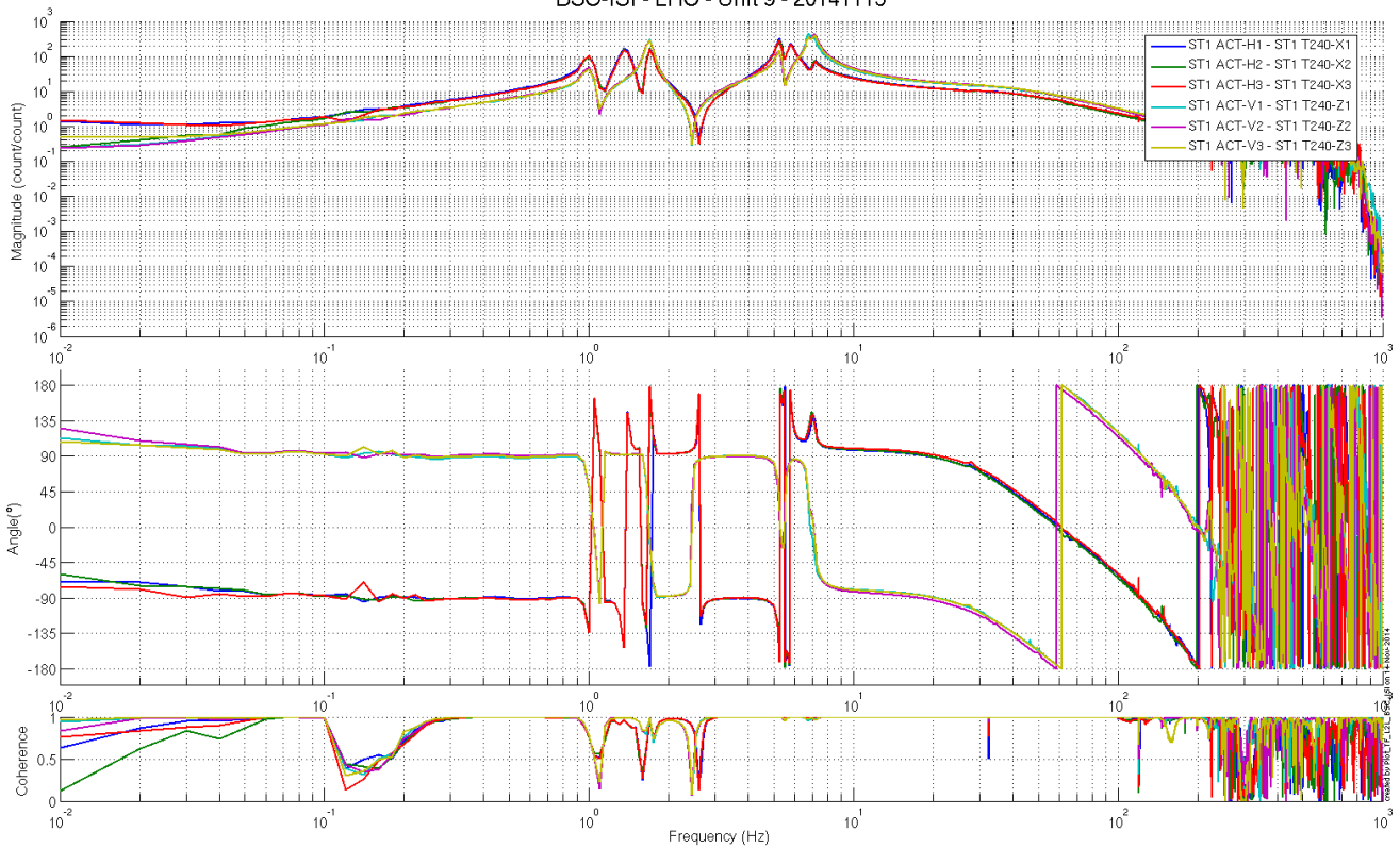
Figure 8 - TF L2L Raw - ST1 Act to ST1 T240 BSC-ISI - LHO - Unit 9 - 20141113
