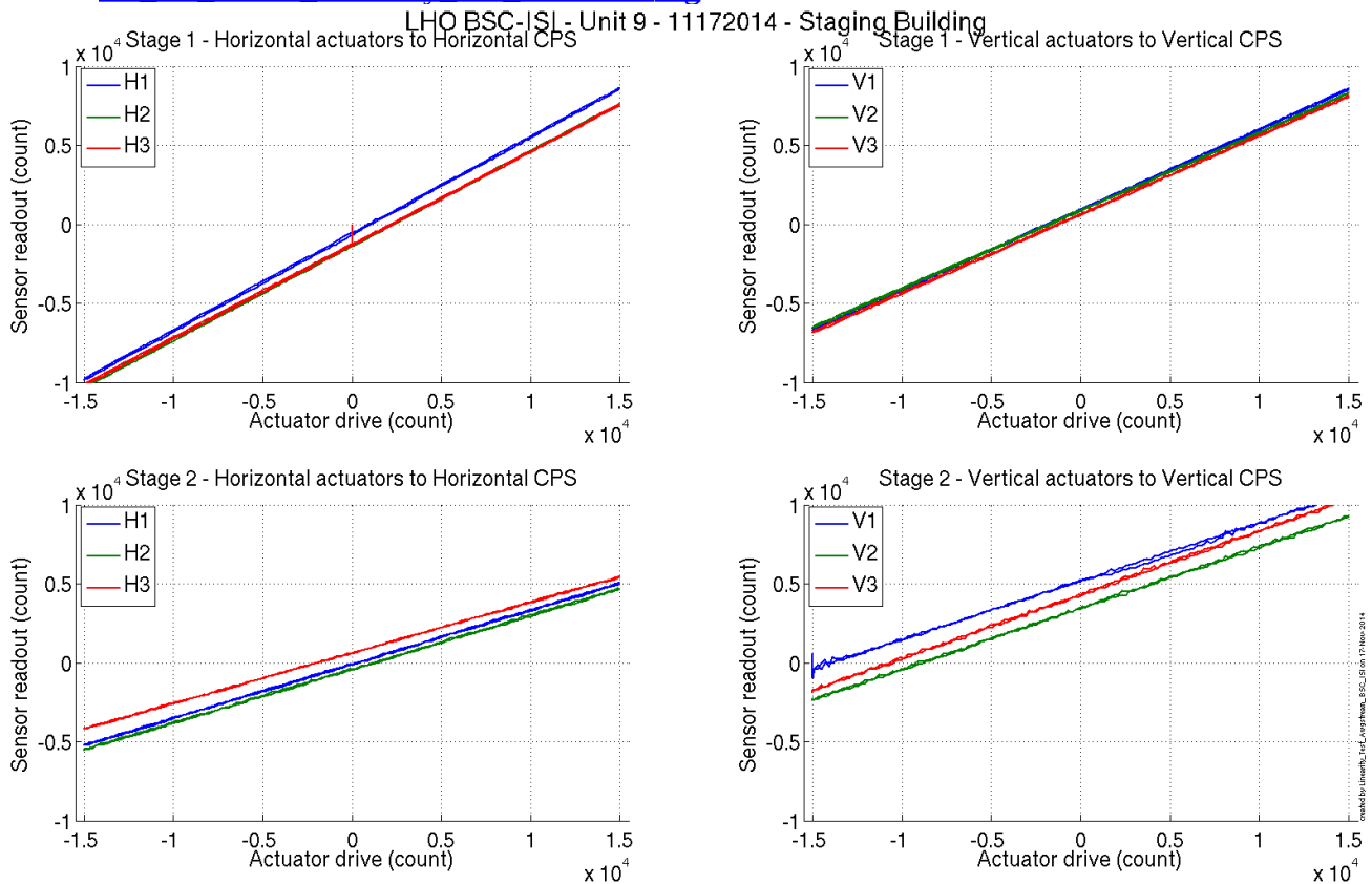
Figure 5 - Linearity Test
