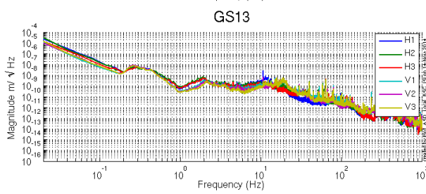
Figure 2: Calibrated Spectra Stage 1 Unlocked and Stage 2 Unlocked
