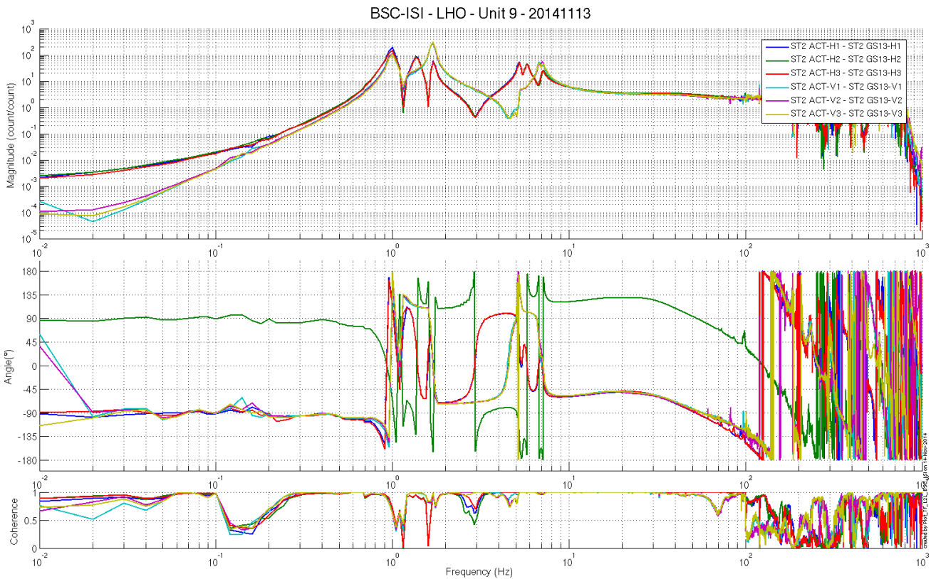
Figure 10: TF L2L Raw - ST2 Act to ST2 GS13
