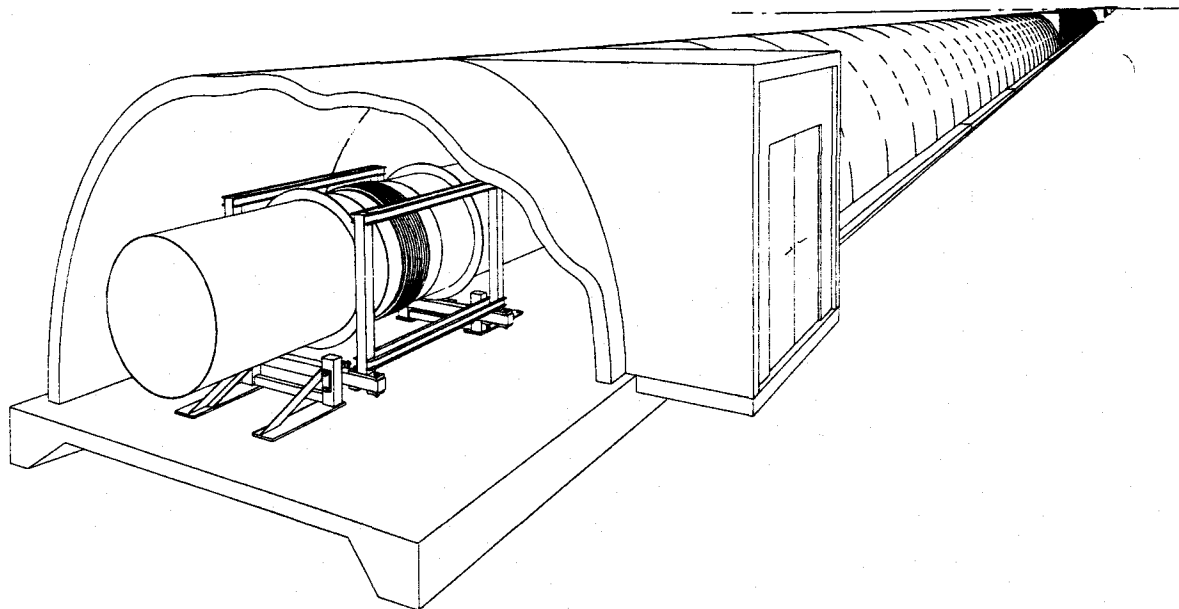
Figure 2.4-1 -- Cut-Away of Beam Tube Enclosure
