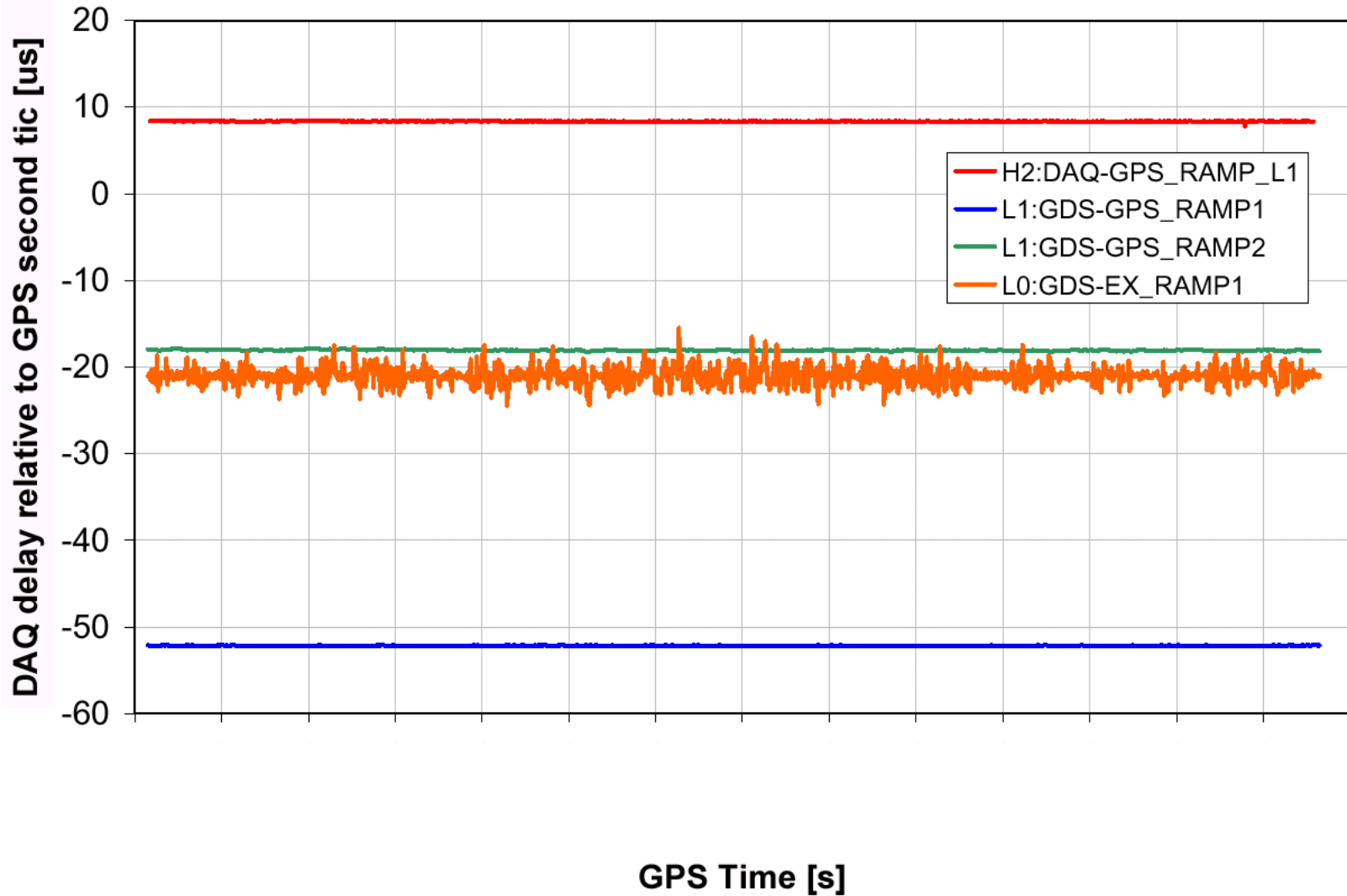
E5 DAQ Timing Shift Trend (Friday-Saturday morning)
