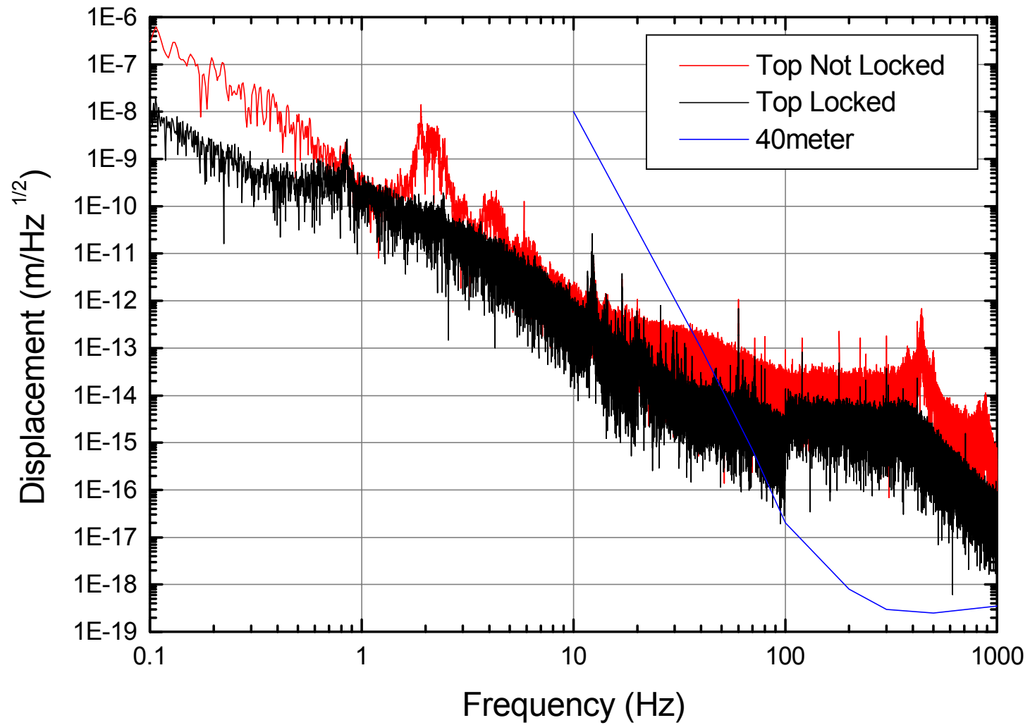
Comparison of Noise spectrum with and without upper interferometer locked 9 March, 2001
