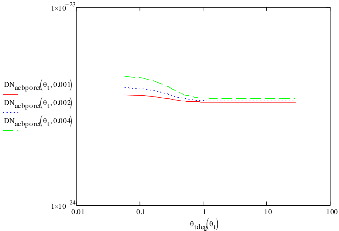
Figure 14: Displacement Noise, Total ACB Scatter, Porcelainized Steel
