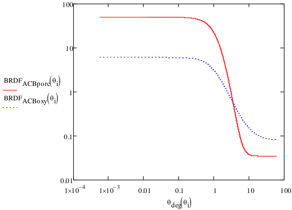
Figure 11: Comparison of #4 Oxidized Polished SS and Porcelainized steel @ 3 Deg Incidence
