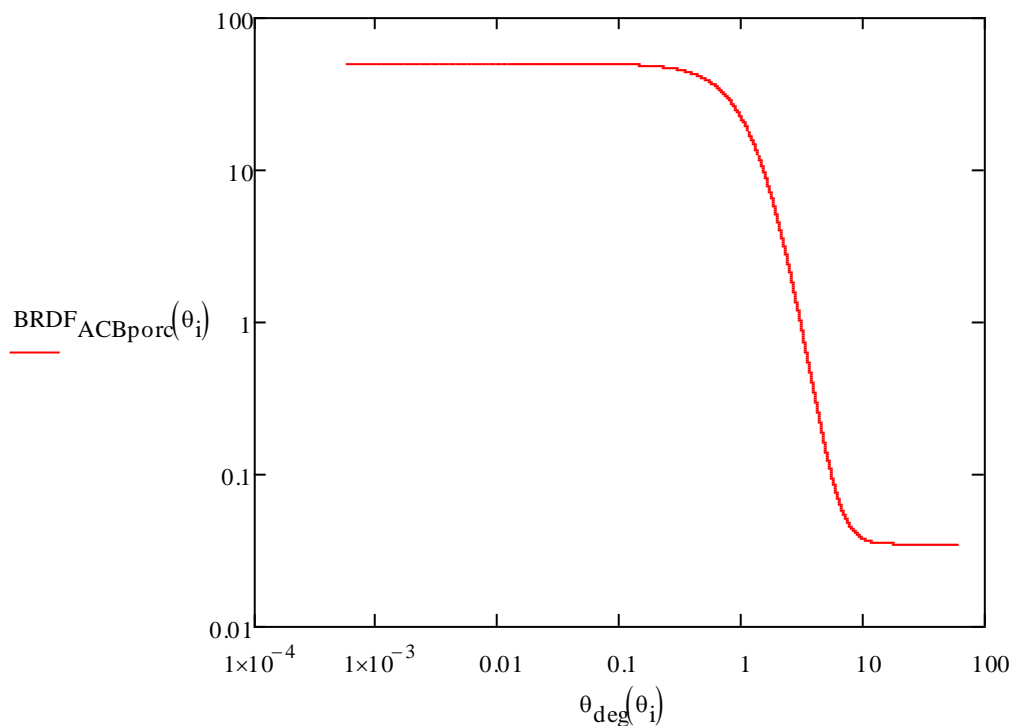
Figure 6: Parametric Equation, Porcelainized Steel BRDF @ 3 deg Versus Scattering Angle Around the Specular Direction
