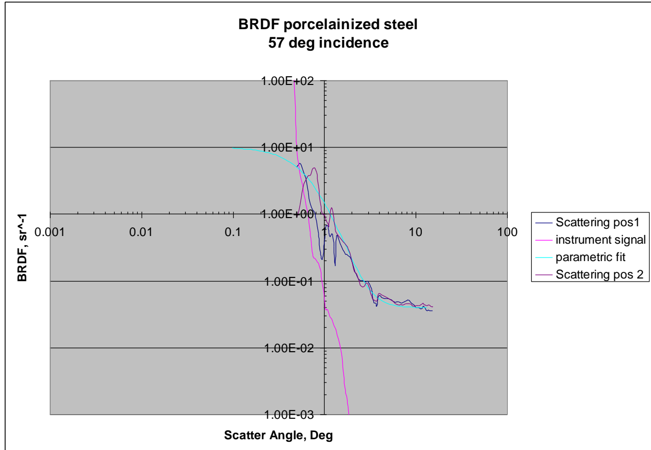
Figure 7: CASI Measurement of BRDF of Porcelainized Steel @ 57 Deg Incidence
