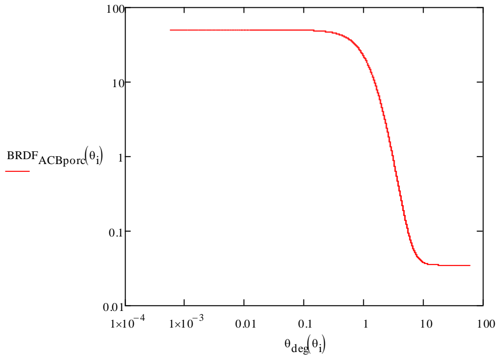
Figure 8: Parametric Equation, Porcelainized Steel BRDF @ 57 Deg Incidence Versus Scattering Angle Around the Specular Direction
