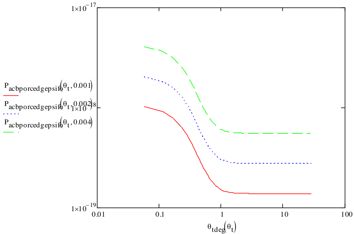
Figure 12: Power Scattered into the IFO Mode from the Baffle Plate Edge, Porcelainized Steel
