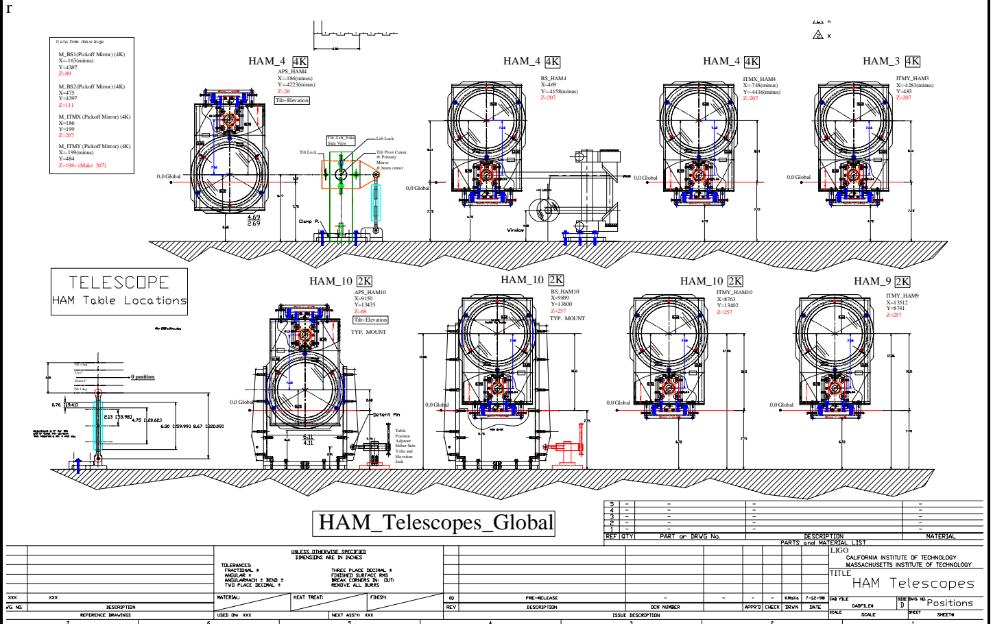
Figure 1: Eight PO Telescope configurations
