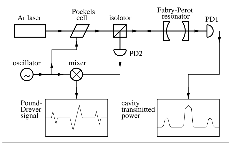
Figure 2: Setup of experiment. The cavity is inside the vacuum envelope which eliminates the fluctuations of the refractive index of air and acoustic coupling of the mirrors.
