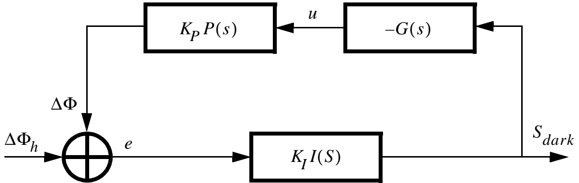
Figure 5: Servo loop model for differential arm length control. The gravitational wave signal \Delta\Phi_h is added to the signal \Delta\Phi coming from the suspended test mass P(s) to give the error signal e which is turned into the antisymmetric port signal S_{dark} by the interferometer I(s) . The controller is described by G(s) and produces the control signal u . The constants K are additional gains; they are mainly introduced to account for gain errors and are nominal unity.
