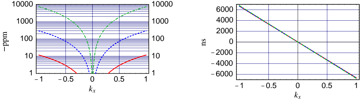
Figure 4: Amplitude correction (left) and time delay of a gravitational wave with non-normal incident and frequencies of 200Hz (solid curve), 1000Hz (dashed) and 5000Hz.
