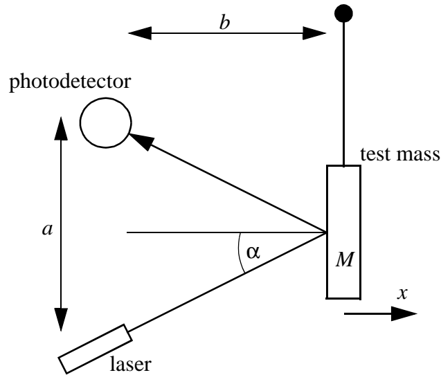
Figure 6: Possible setup of a photon actuator.
