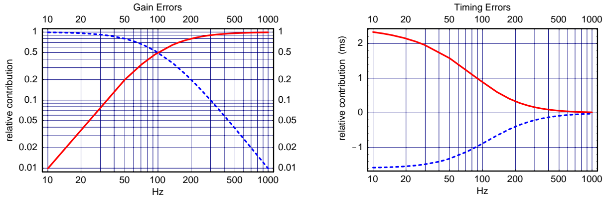
Figure 8: Relative contribution of an error in K_I (solid curve) and K_P to the gain error (left) and to the timing uncertainty. The unity gain frequency was chosen at 100Hz.
