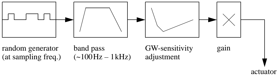
Figure 7: Pseudo-random signal generation.
