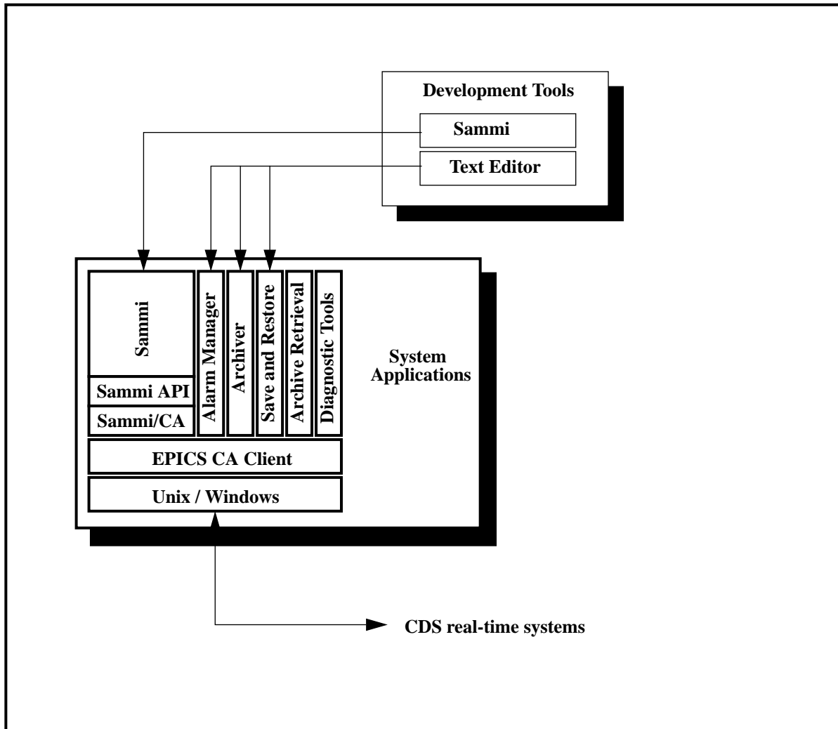
Figure 24: Non-real-time Software Overview
