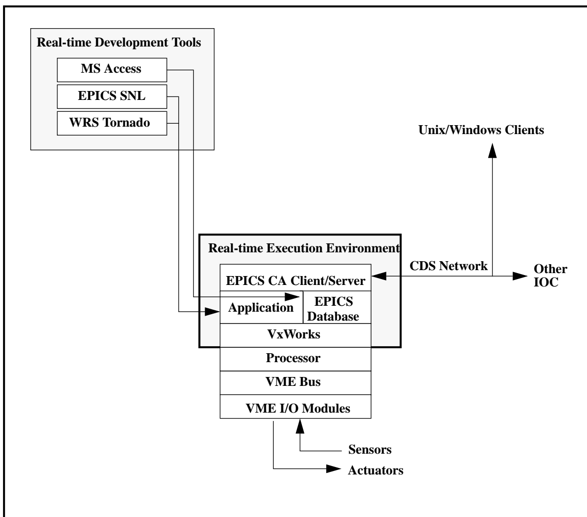
Figure 21: Real-time Software Overview
