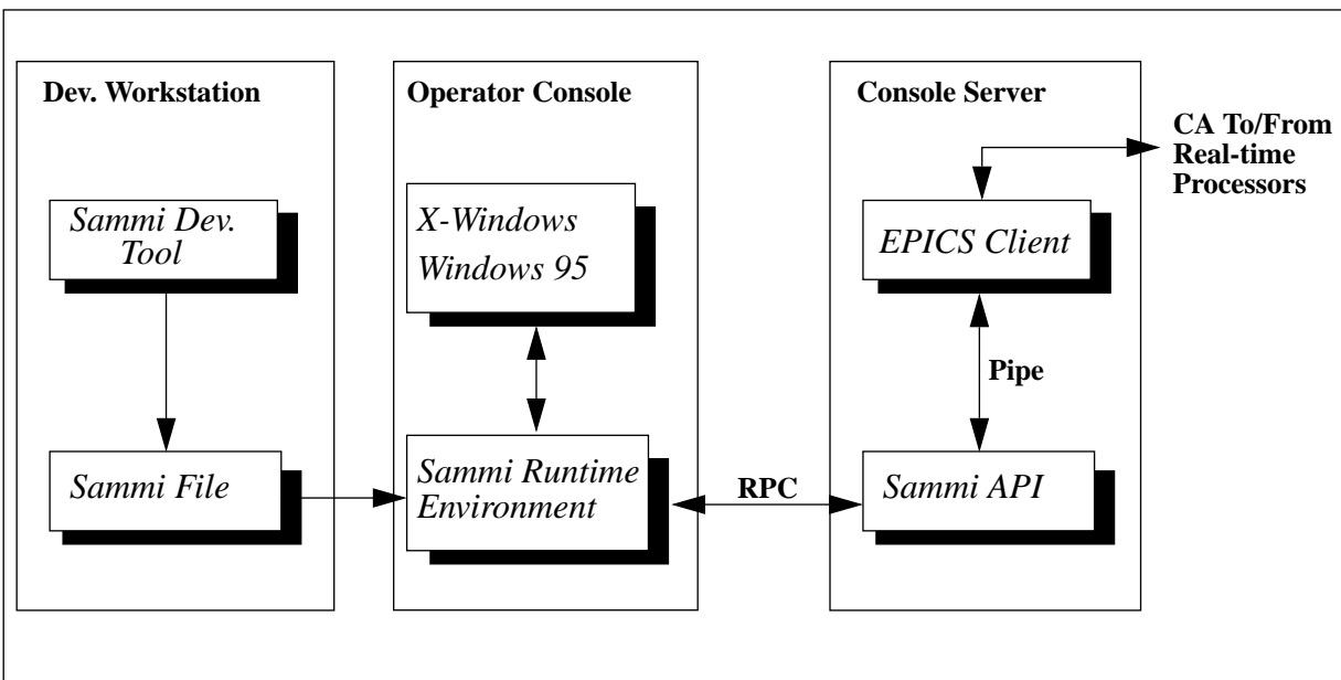
Figure 25: HMI to CDS Real-time Connection
