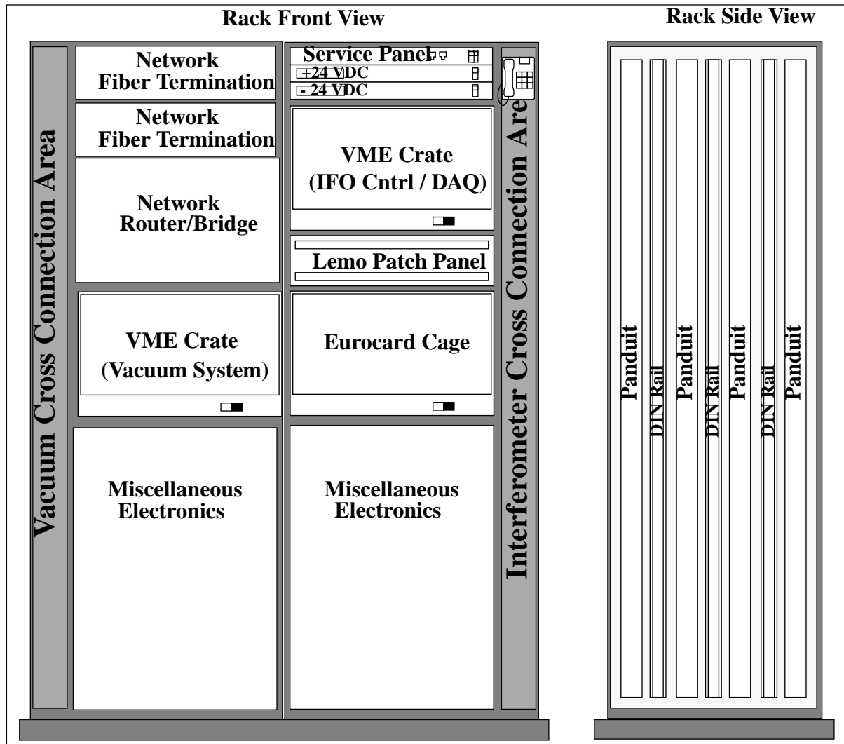
Figure 6: Standard Rack Layout (Mid and End Stations)
