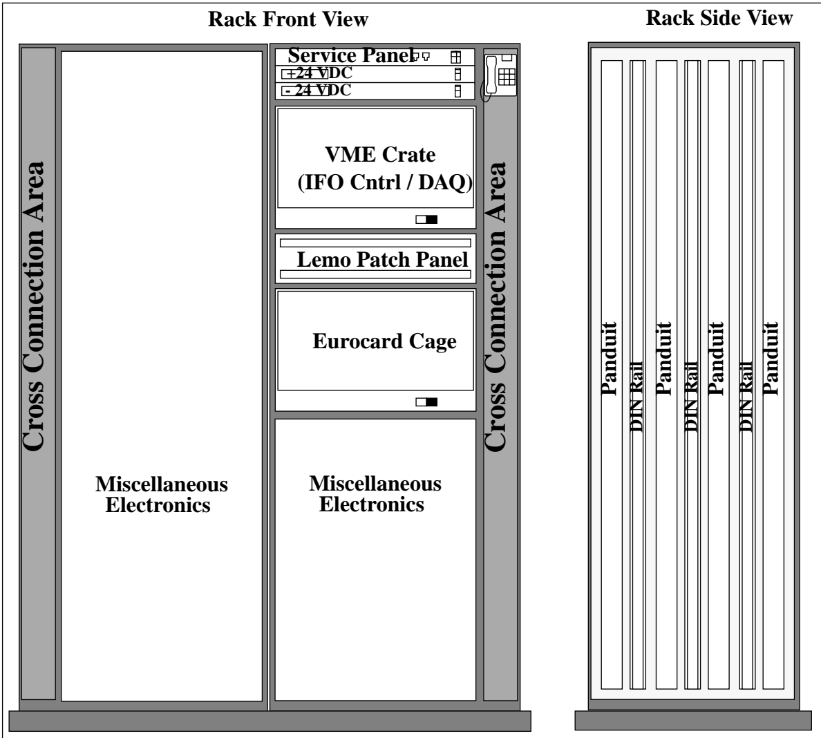
Figure 5: CDS Standard Front End Rack Assembly (LVEA)
