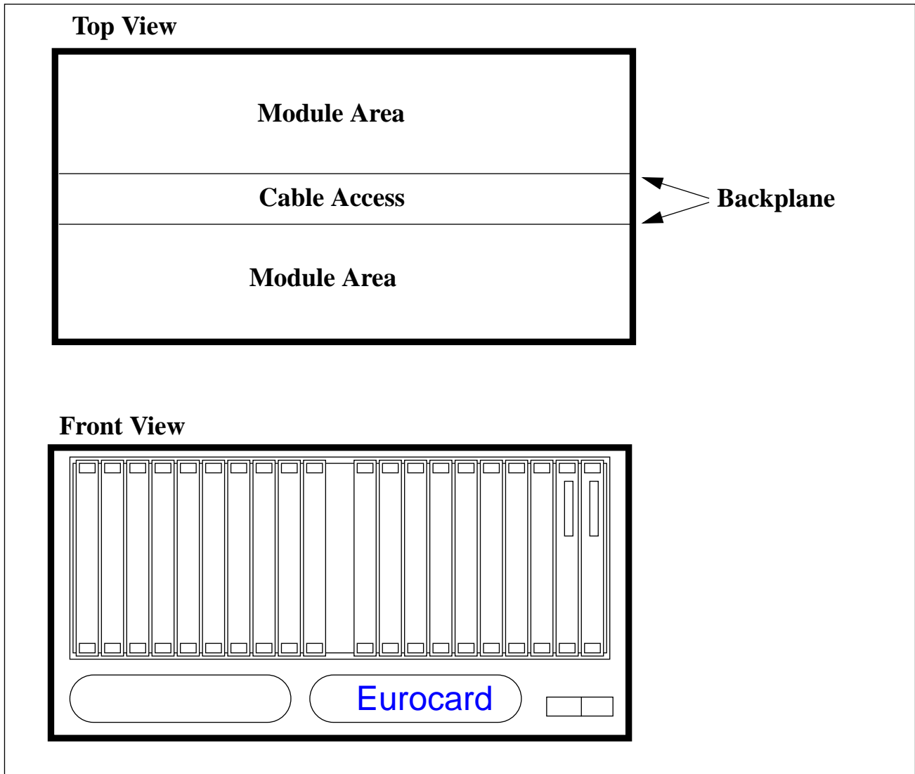
Figure 3: CDS Eurocard Cage
