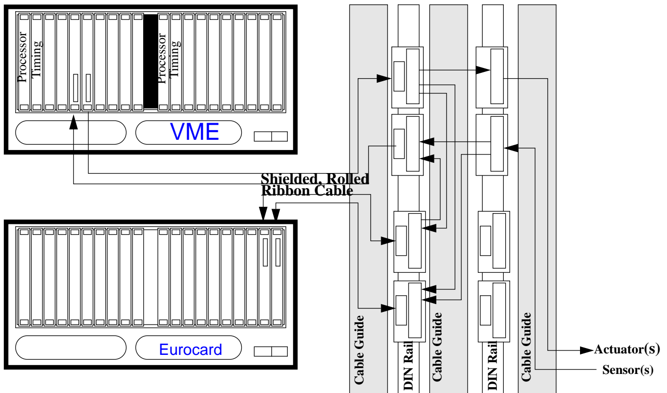
Figure 7: CDS Cable Interconnect System
