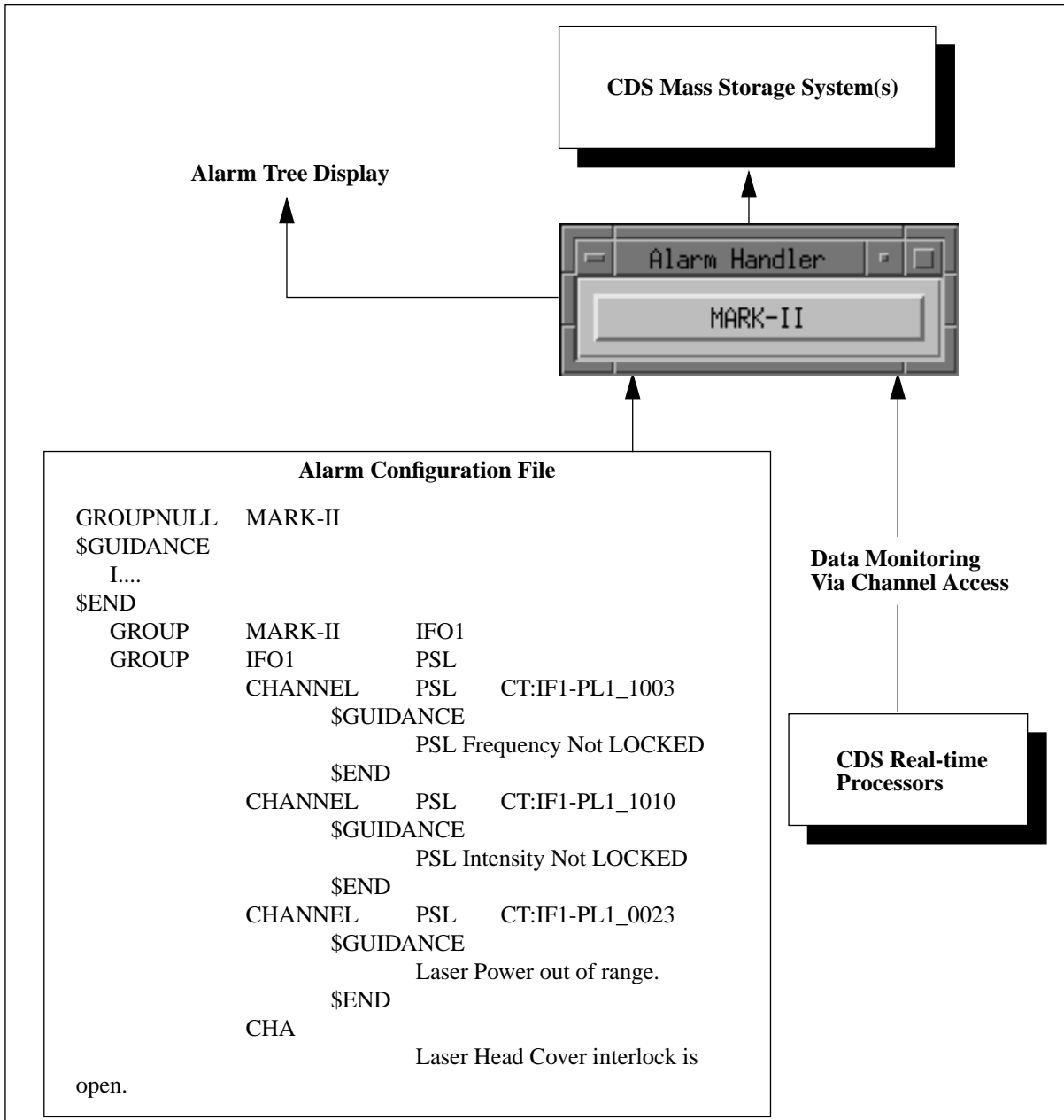
Figure 28: Alarm Management Software Architecture
