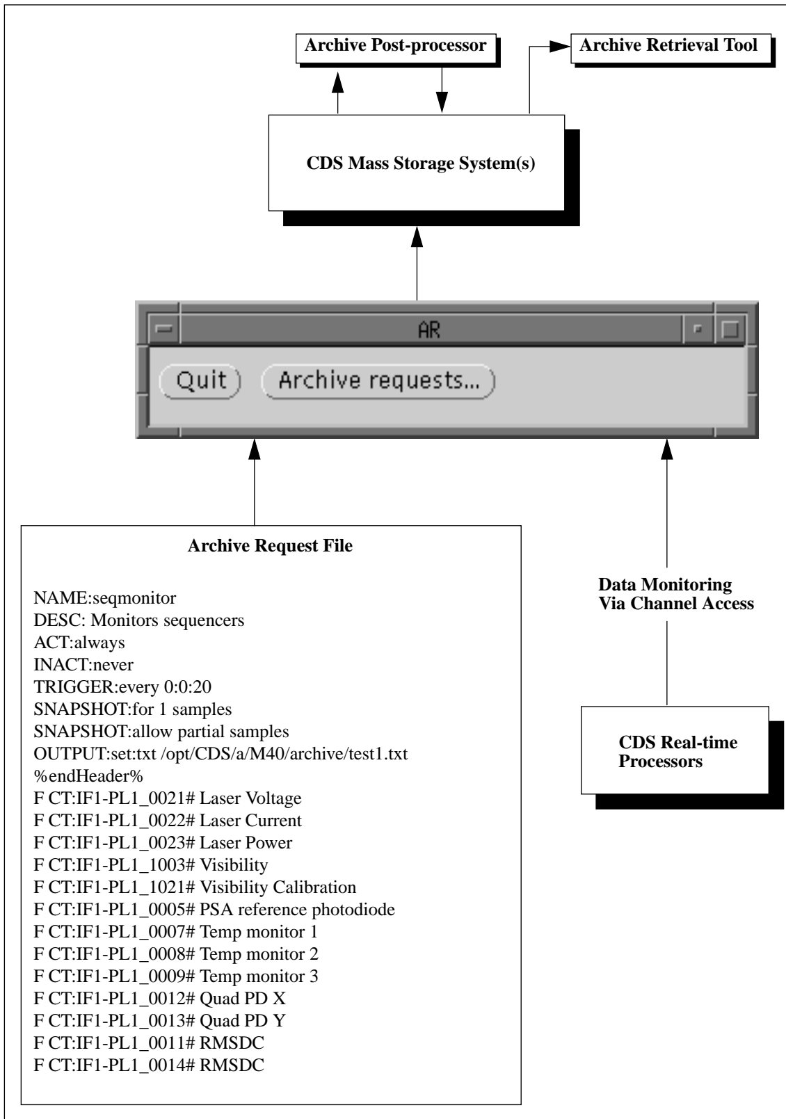
Figure 26: Data Archive Software Structure
