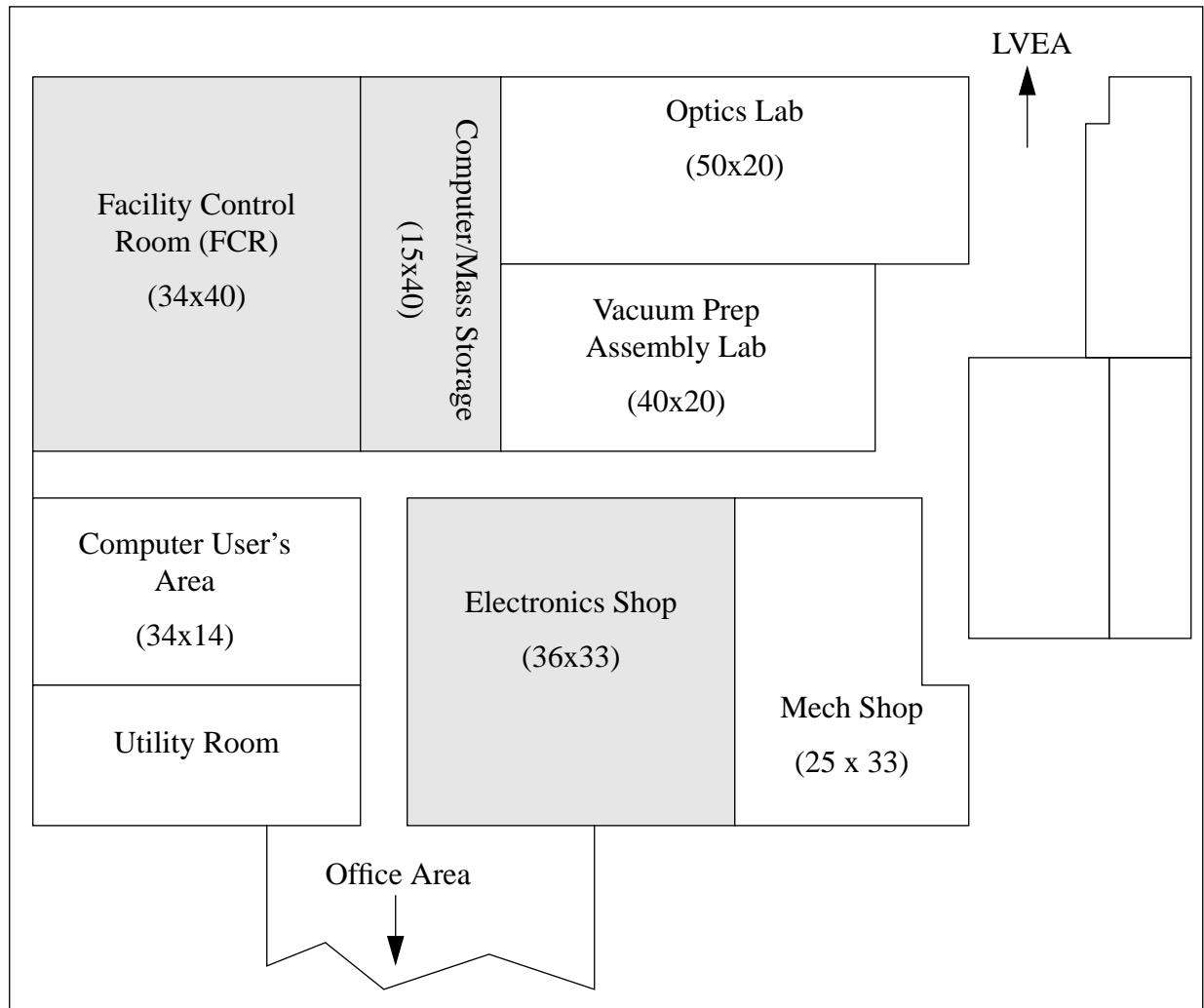
Figure 14: OSB Conceptual Design (Partial)
