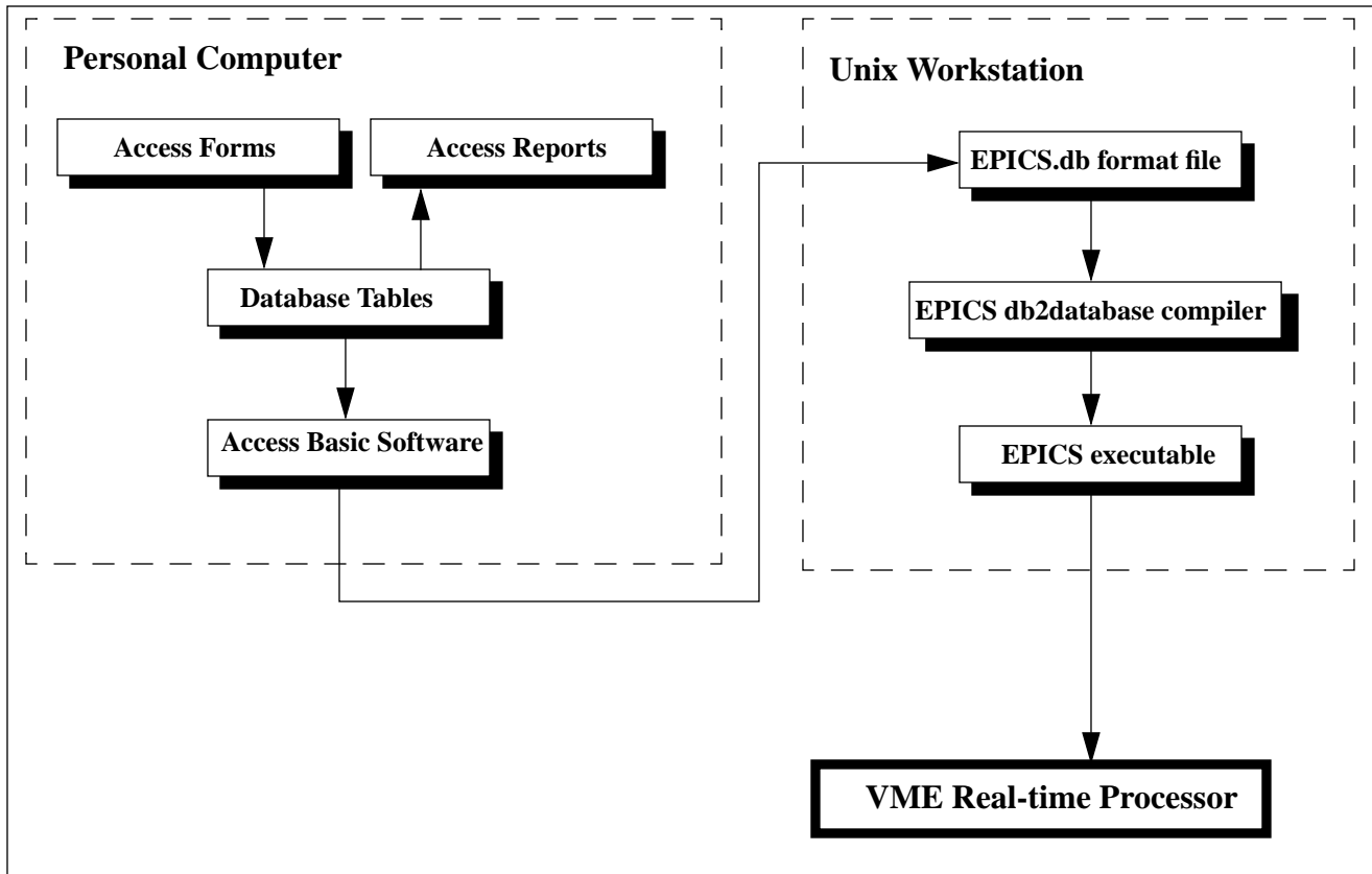
Figure 23: MS Access to EPICS Database
