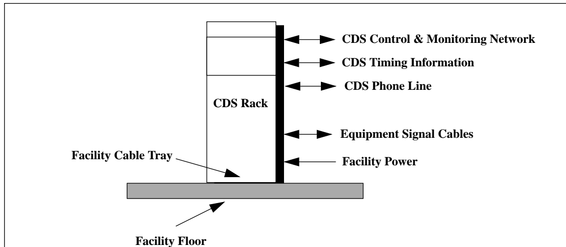
Figure 8: CDS Front End Rack Interfaces
