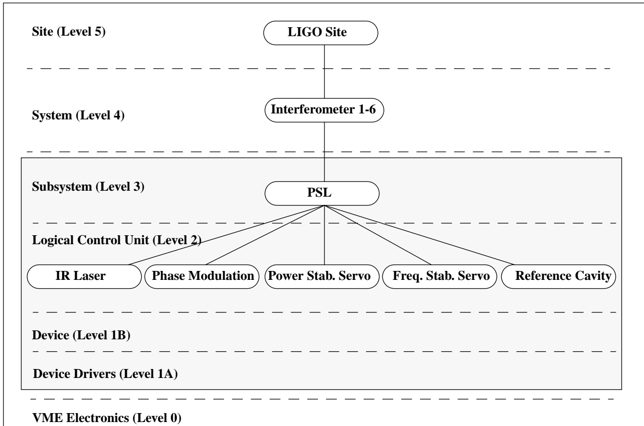
Figure 20: PSL CIM Model Example
