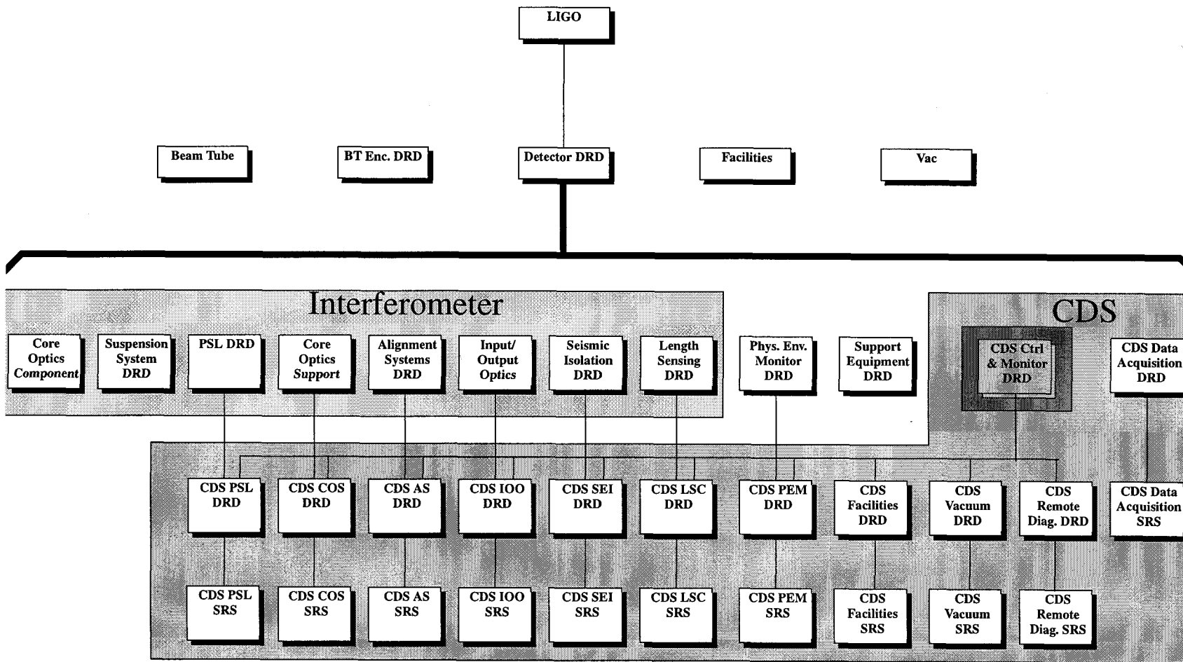
Figure 1: LIGO Detector Requirement Specification Tree
