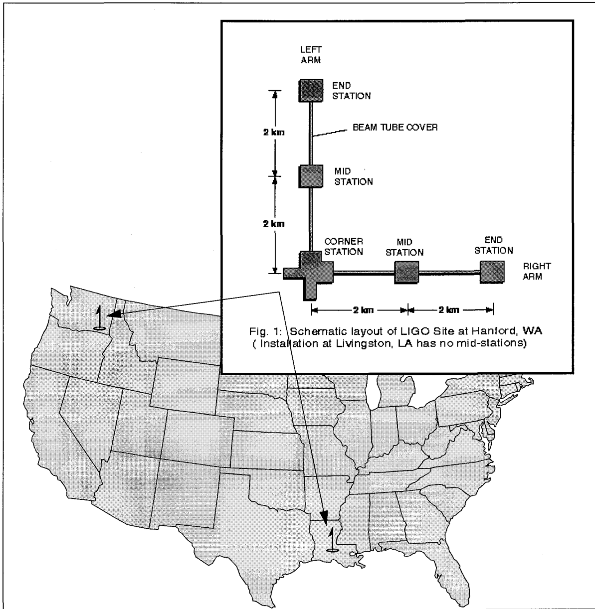
Figure 4: LIGO Site Overview
