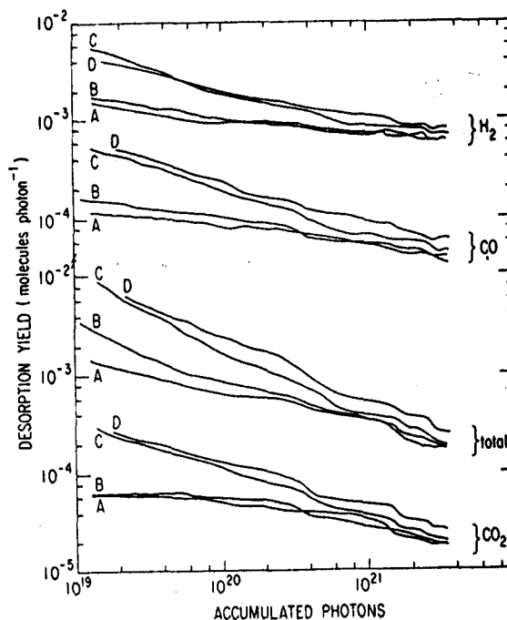
FIG. 5. Photodesorption yields of the samples after different degassing treatments: (A) chemical cleaned, vacuum fired, and GDC; (B) chemical cleaned, vacuum fired, and NO treated; (C) chemical cleaned and vacuum fired; and (D) chemical cleaned. The accumulated photons are those over an area of \sim 20 cm 2 .
