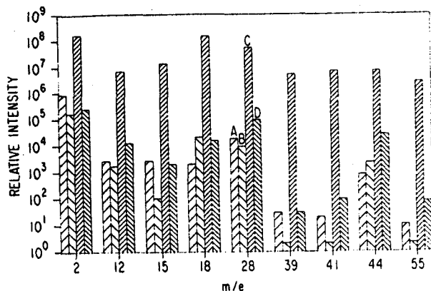
FIG. 2. The variation in residual gas composition before and after NO treatment. A and B are those of a clean chamber before and after the treatment, respectively; C and D are those of contaminated chamber before and after NO treatment.
