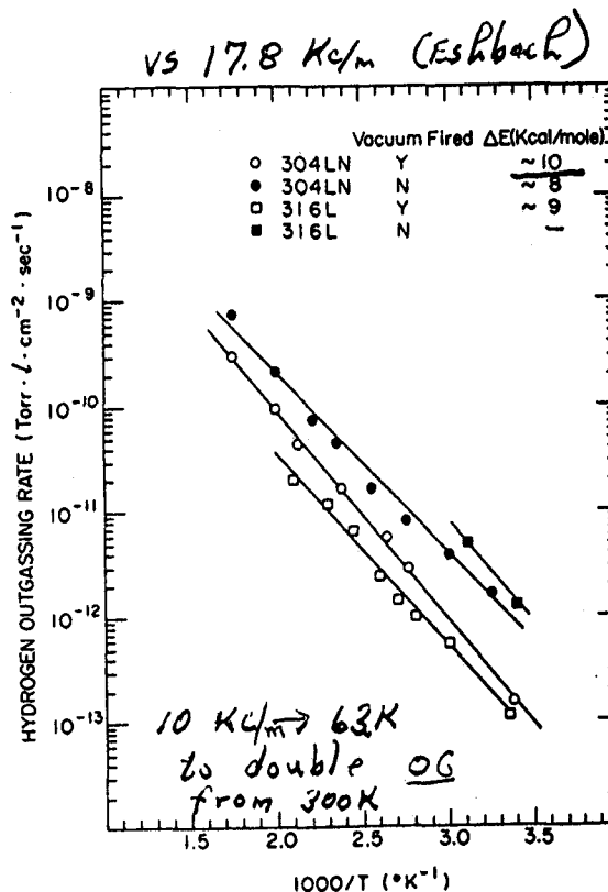
FIG. 4. The outgassing rates of hydrogen for the 304LN and 316L stainless-steel vacuum chambers at different temperatures. The enthalpy ΔE is the least-square fit of the data to Q = Q 0 exp(-ΔE/RT).
