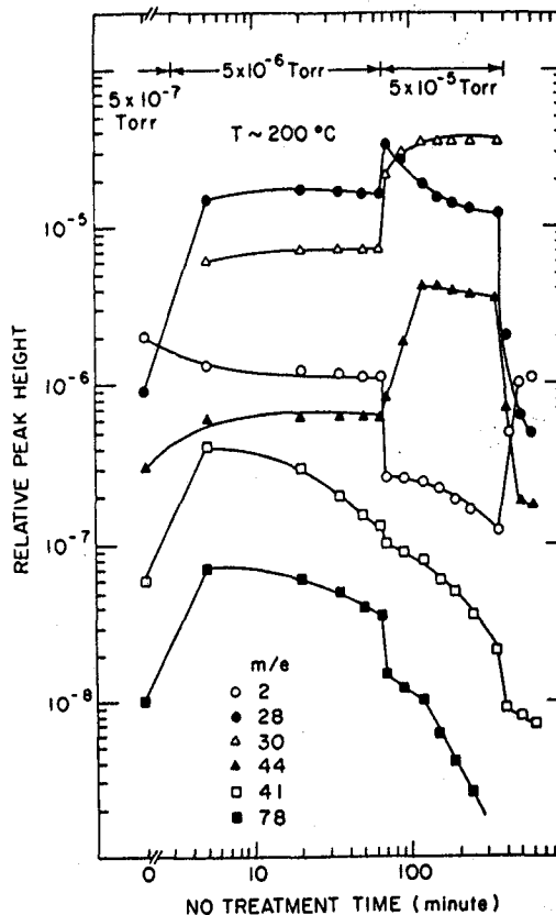
FIG. 1. Typical residual gas composition during nitric oxide treatment of a test chamber which was chemical cleaned and vacuum fired. The chamber was maintained at 200 °C. The NO pressure was either 10 or 100 times the background pressure. The lines are for guiding the eyes.
