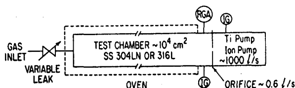
FIG. 3. Experimental setup for measuring the thermal outgassing rate of the long vacuum chambers.
