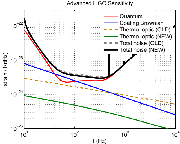
Figure 3: An Advanced LIGO sensitivity curve. The thermo-optic curve labeled “NEW” uses equation 50, while the “OLD” curve uses a conservative estimate of TO noise: the sum of TR and TE, with the TE correction factor of 1.56 from [7].
