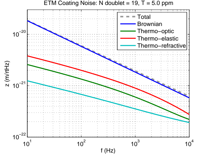
Figure 2: Thermo-optic noises and Brownian noise for an Advanced LIGO end mirror.
