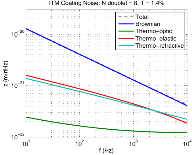
Figure 1: Thermo-optic noises and Brownian noise for an Advanced LIGO input mirror.
