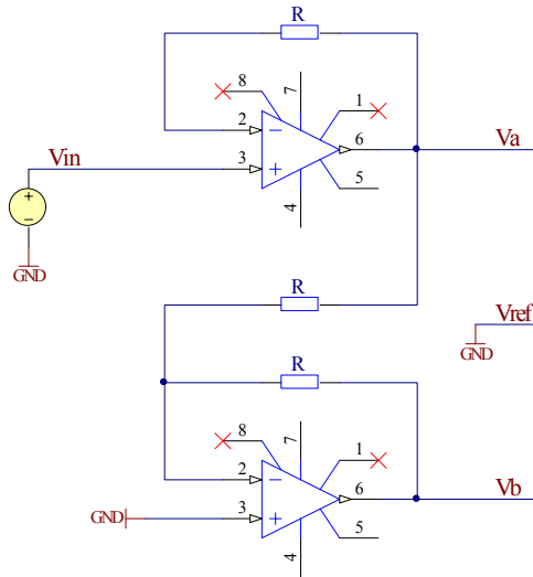
Differential Driver
