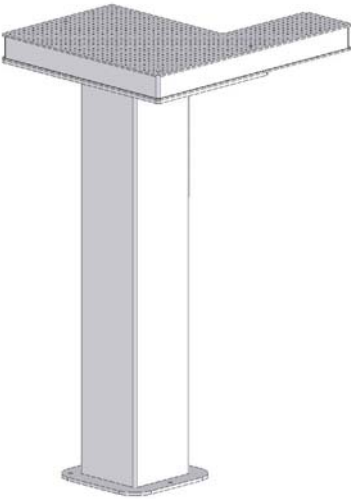
Figure 5 Pcal support structure – breadboard and pier.
