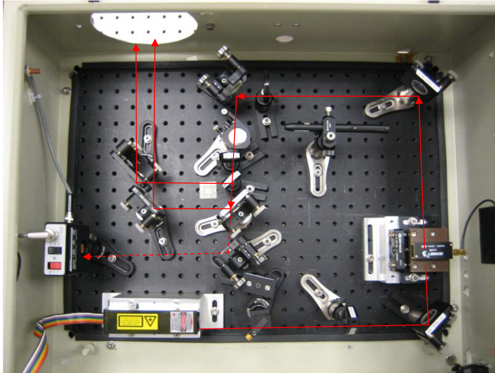
Figure 3 Bird's-eye view of proposed layout upgrade. The two-beam output configuration is shown. The horizontally-polarized laser output passes through a polarizing beamsplitter cube before being focused into the AOM. The first order diffracted beam is then focused by a single spherical lens on the way to a 50% beamsplitter. The splitting ratio is fine tuned by adjusting the angle of incidence by rotating the splitter. The reflected and transmitted beams are then directed to the final steering mirrors that control the beam positions on the ETM. The PD would be replaced by an integrating sphere with an integrated PD if the proposed power monitoring upgrade is implemented. The laser pointer and flipper mount are for initial rough alignment of both beams.
