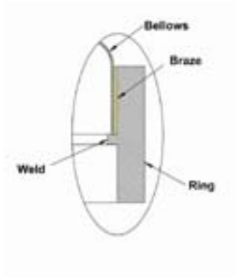
Braze Joint A detail.jpg
