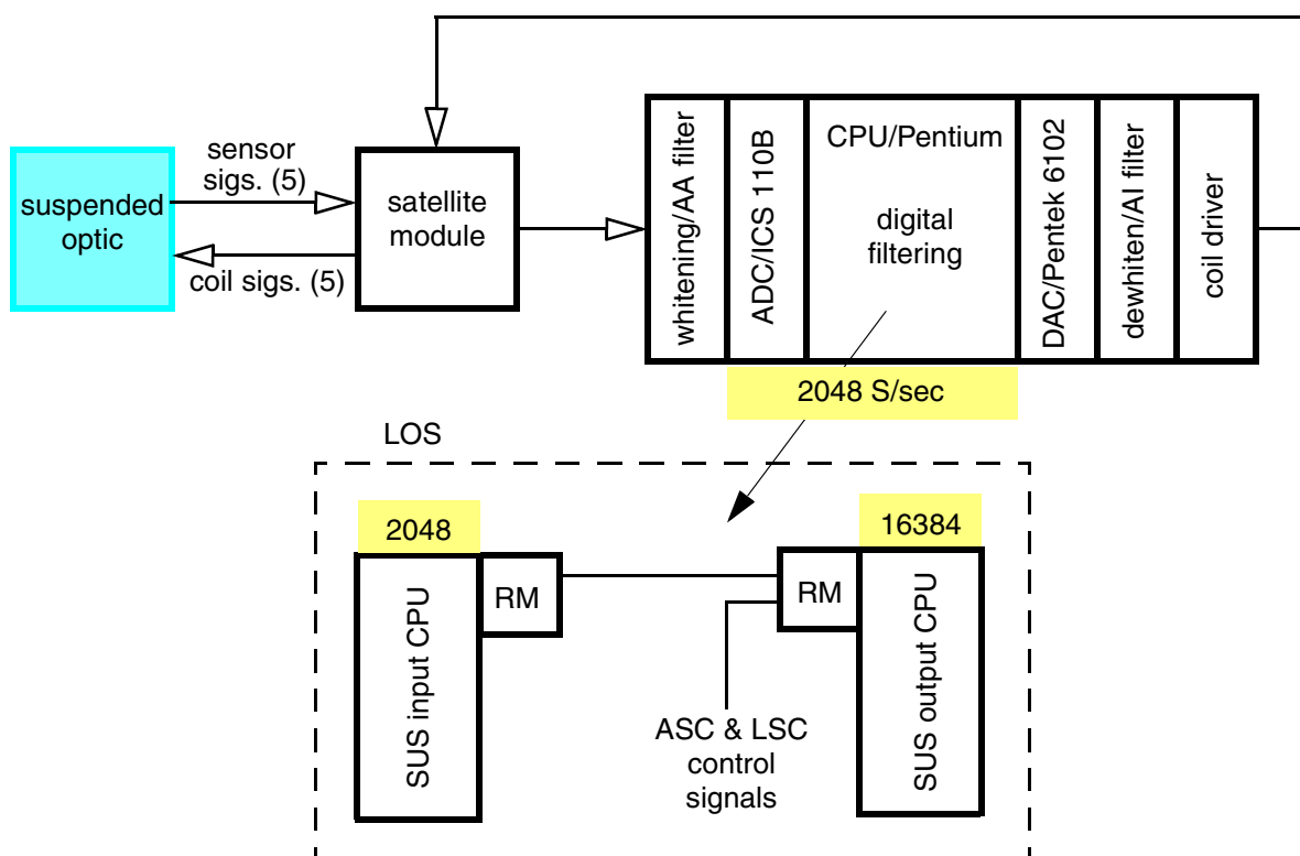
Figure 1. Block diagram of the digital suspension system. For the SOS, a single Pentium CPU processes all suspension signals. For the LOS, one Pentium CPU processes the suspensions' local sensor signals (SUS input CPU), and a second CPU combines these suspension signals with the ASC & LSC signals and performs appropriate output processing (SUS output CPU). The second CPU calculates at the LSC rate of 16,384 S/sec
