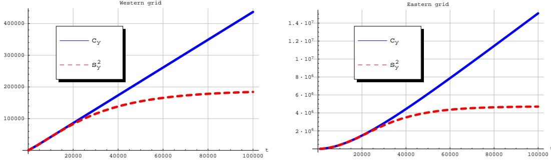
Figure 11: The comparison between the exact form of the structure function E [(\psi(t) - \psi(t_0))^2] for the process \psi and the approximation c_\psi(t - t_0) . The plot at left is obtained with the values appropriate for the Western grid, while the plot at right is appropriate for the Eastern grid
