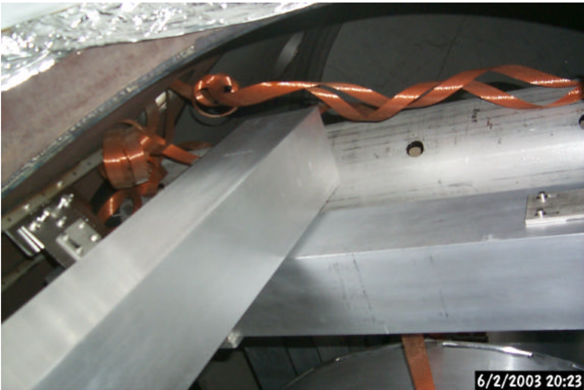
BSC7 COS cavity beam dump tubes and LOS ribbon cables, as viewed from below, standing at East door.
