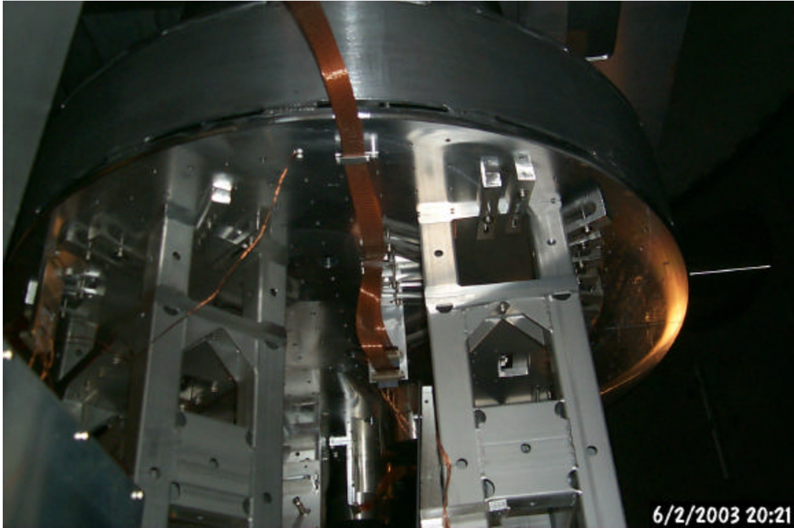
New 2k ITMx LOS on right, FMx on left.
