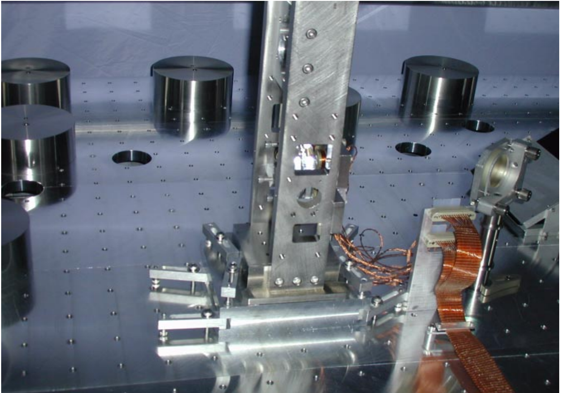
HAM2 MMT2 viewed from East Side.
