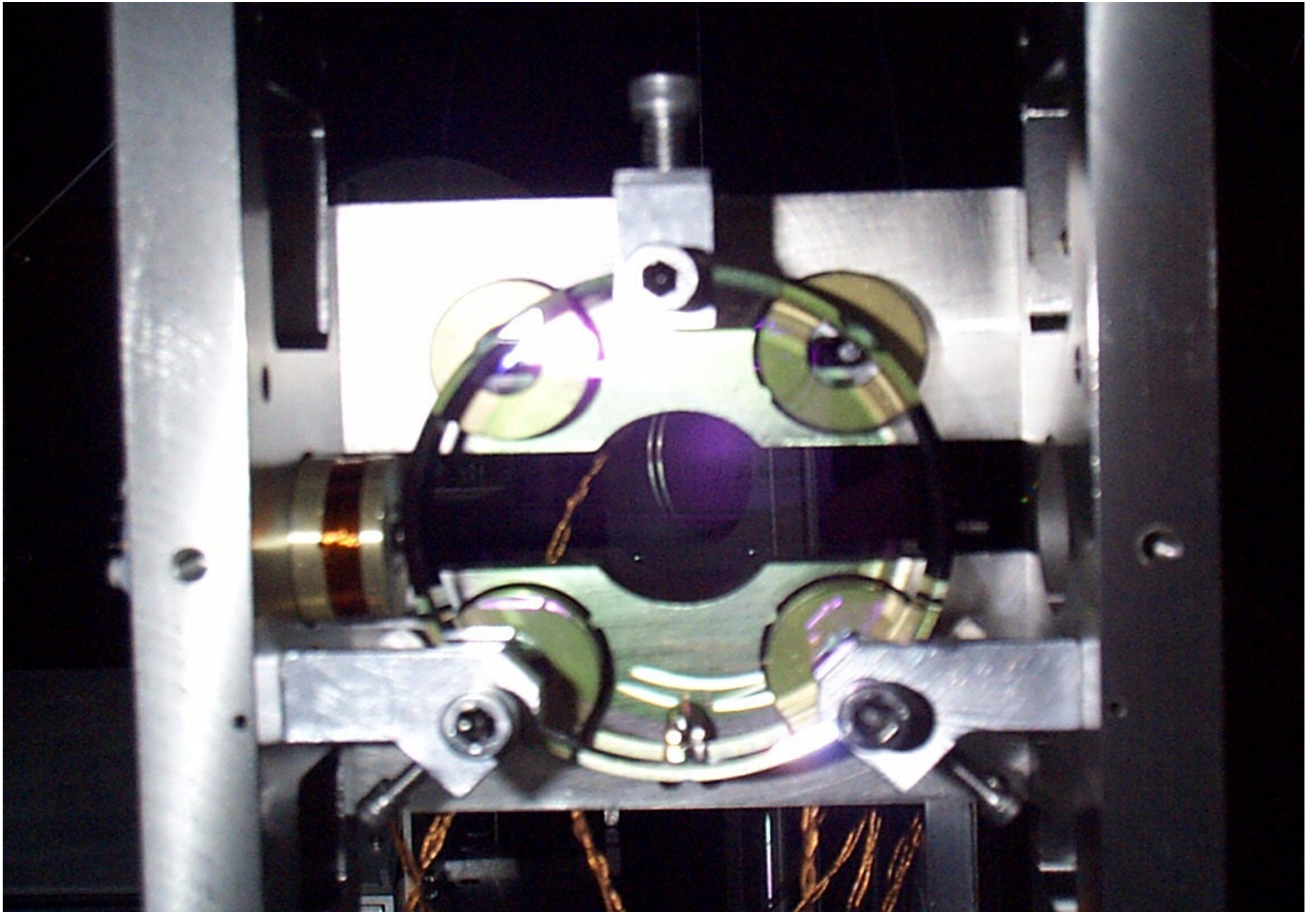
HAM2 MMT2 Optic Front Closeup
