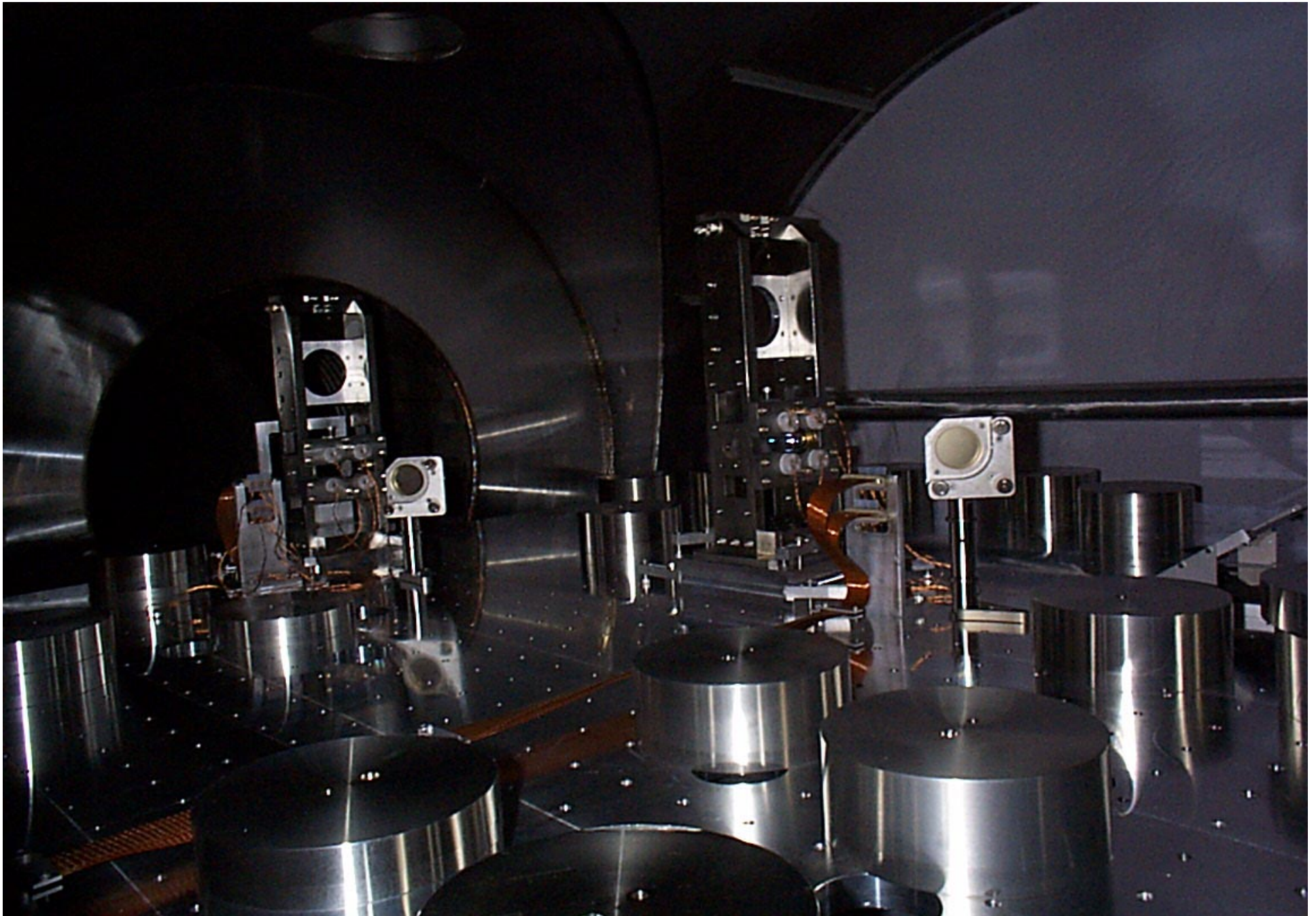
HAM2 Looking SW at the backs of MMT2 (right) and MC2 (left).
