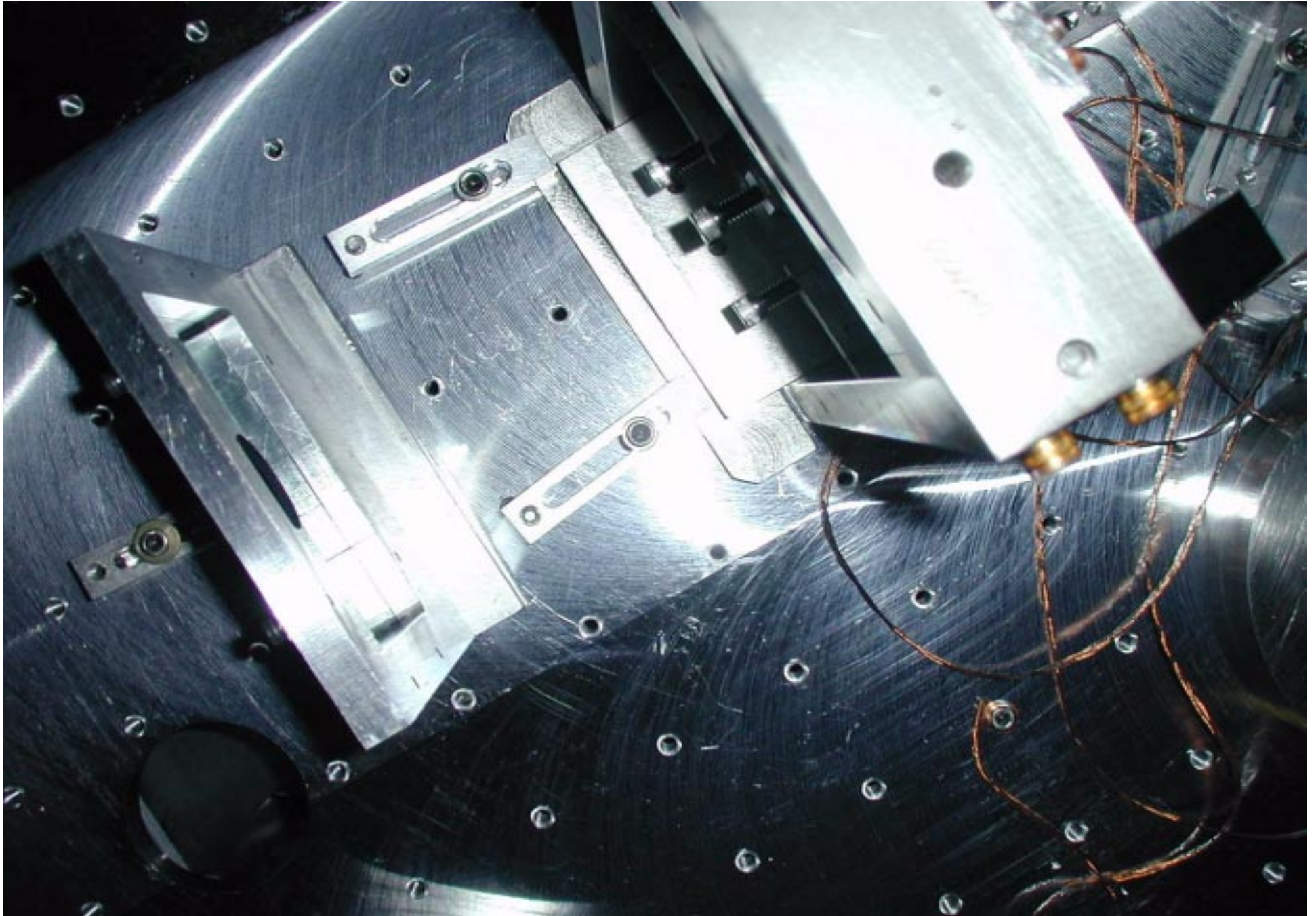
HAM2 Top down view of MC2 Baffle (left) and MC2 (right), NE is to the right.
