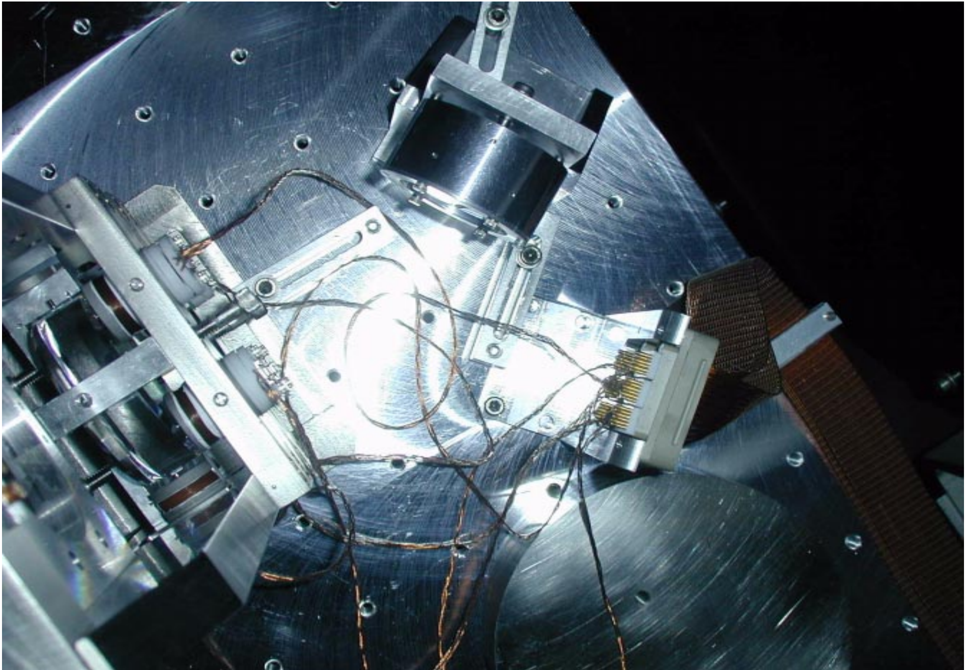
HAM2 Top down view of MC2 (left), optical lever steering mirror (top right) and OSEM cable connector (bottom right)
