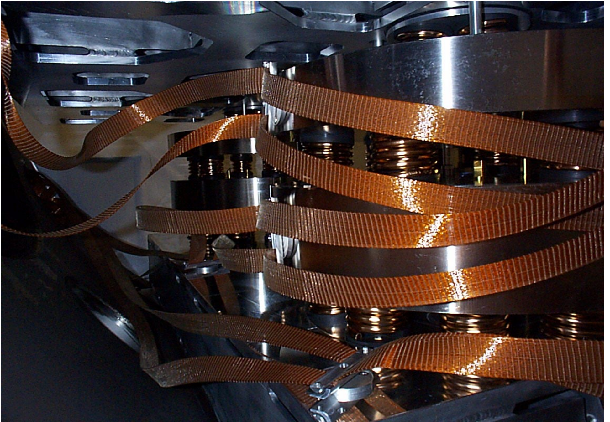
HAM2 SE stack in front field and SW stack in background, viewed from SE
