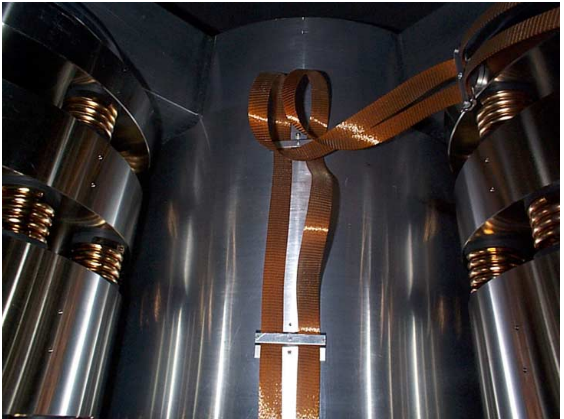
WBSC 6 Mar 1, 2000: 226. NW stack, from N; post tuning
