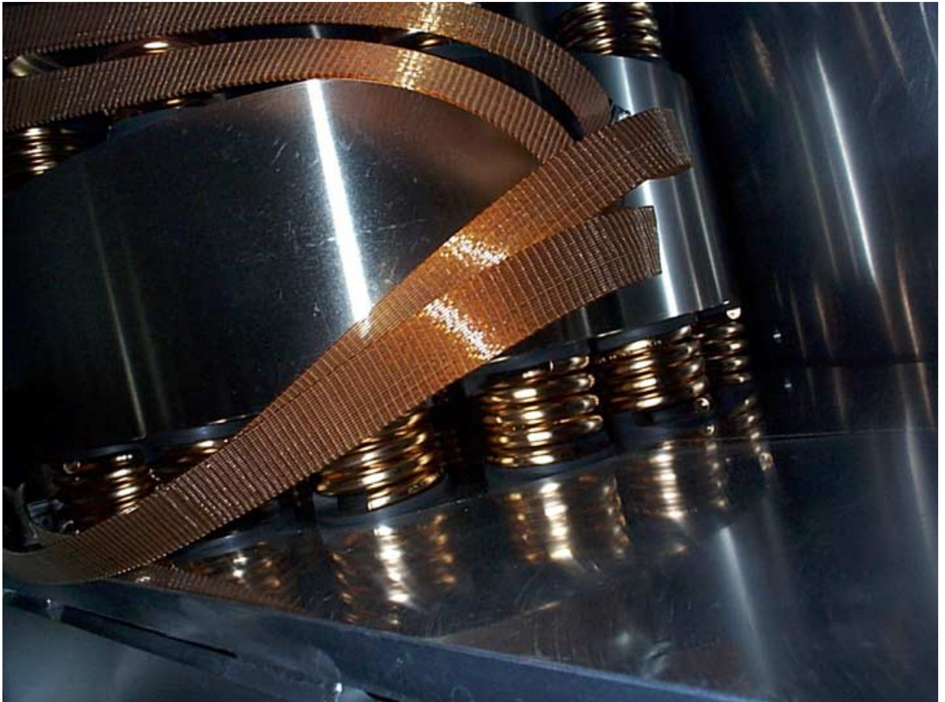
WBSC 6 Mar 1, 2000: 232. NW stack, from W; post tuning attempt
