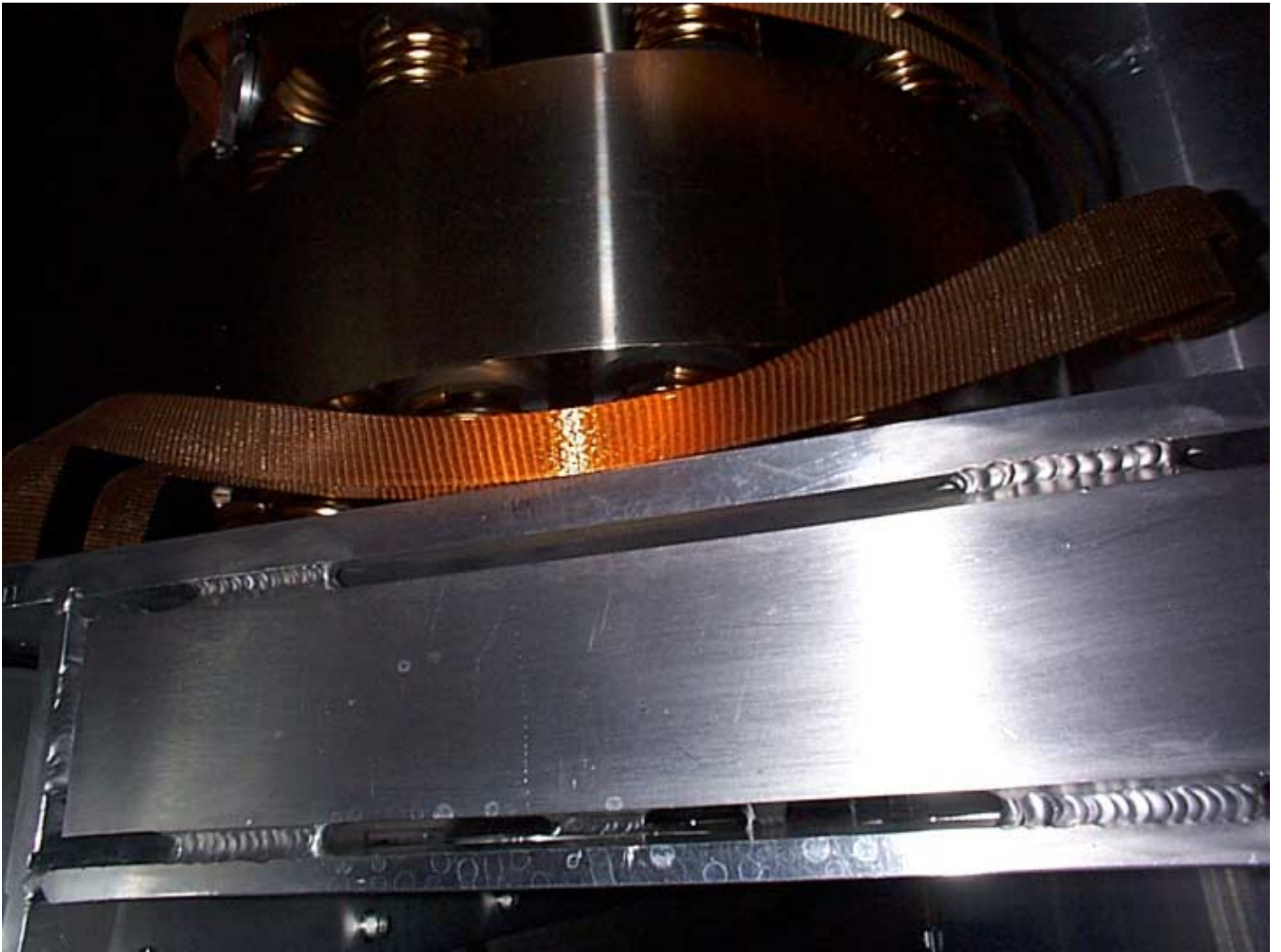
WBSC 6 Feb 29, 2000: 223. NW stack, from W; cable is touching table
