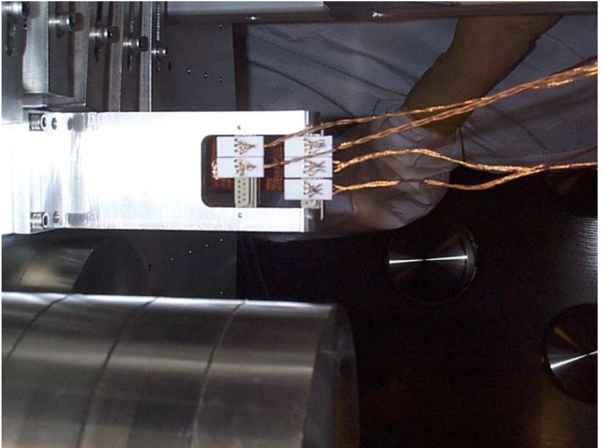
WBSC 6 Feb 29, 2000: 221. ETMy cable termination bracket
