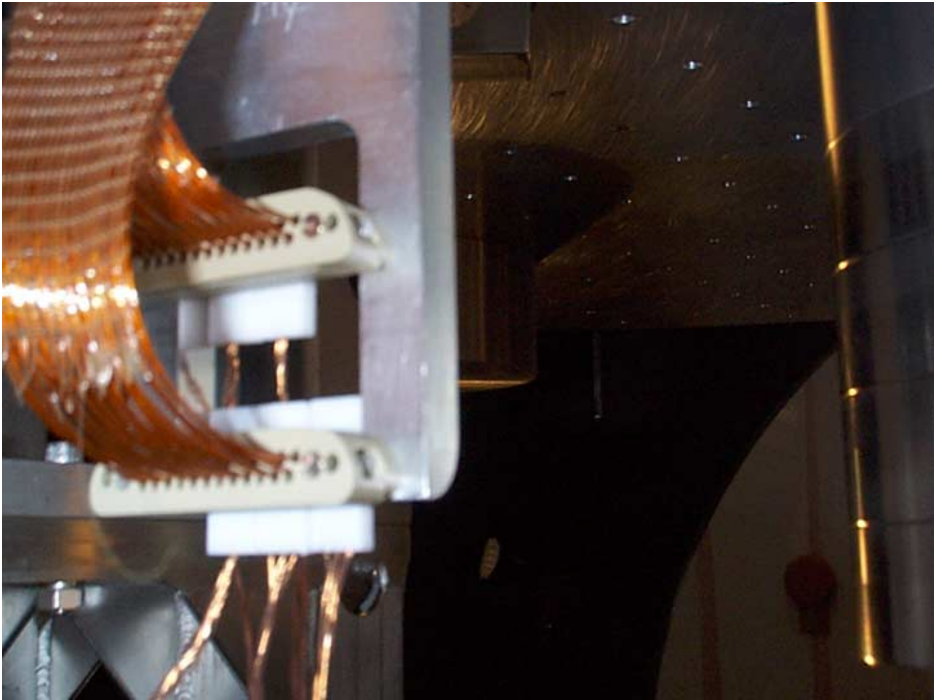
WBSC 6 Feb 29, 2000: 220. ETMy cable termination bracket
