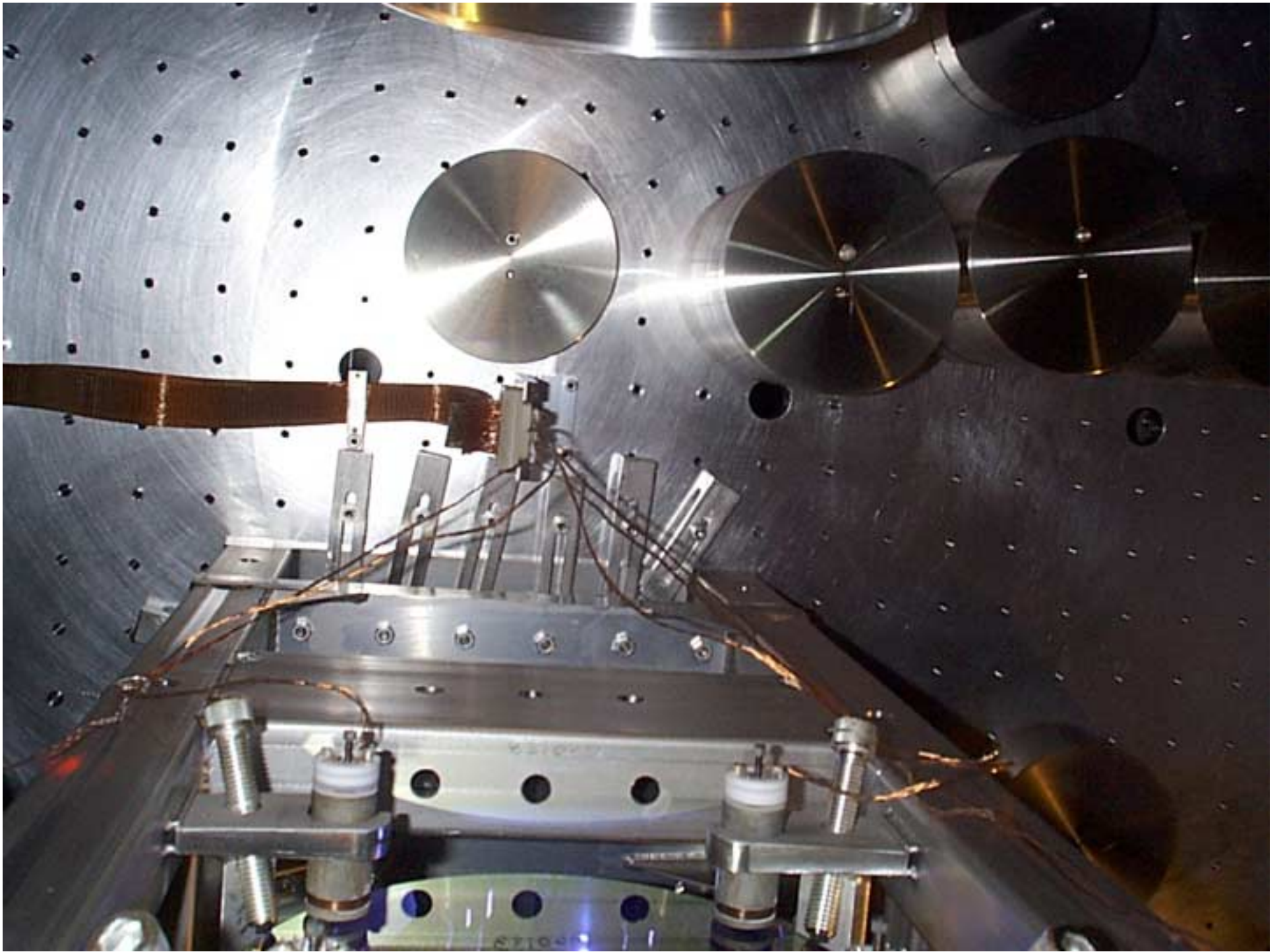
WBCS 6 Feb 29, 2000: 218. +Y @ top
