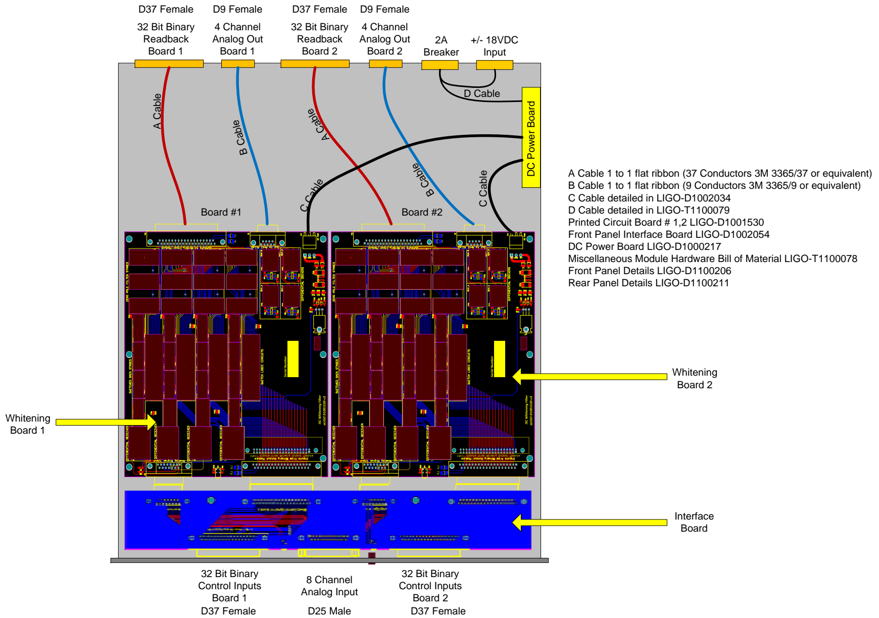
ISC 8 Channel Whitening Chassis Assembly Drawing D1002559-v3
