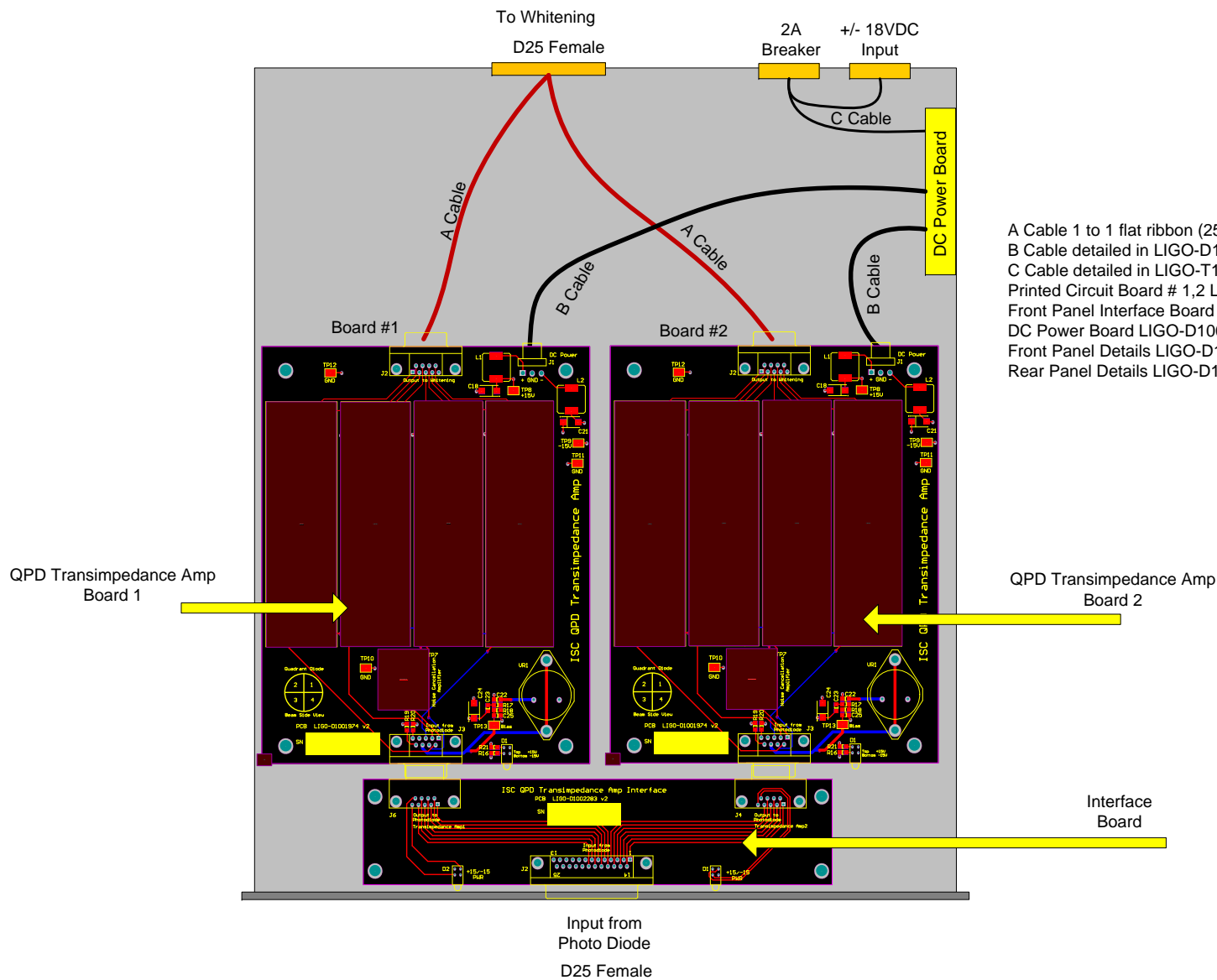
ISC Dual QPD Transimpedance Amplifier Chassis Assembly Drawing D1002481-v2
