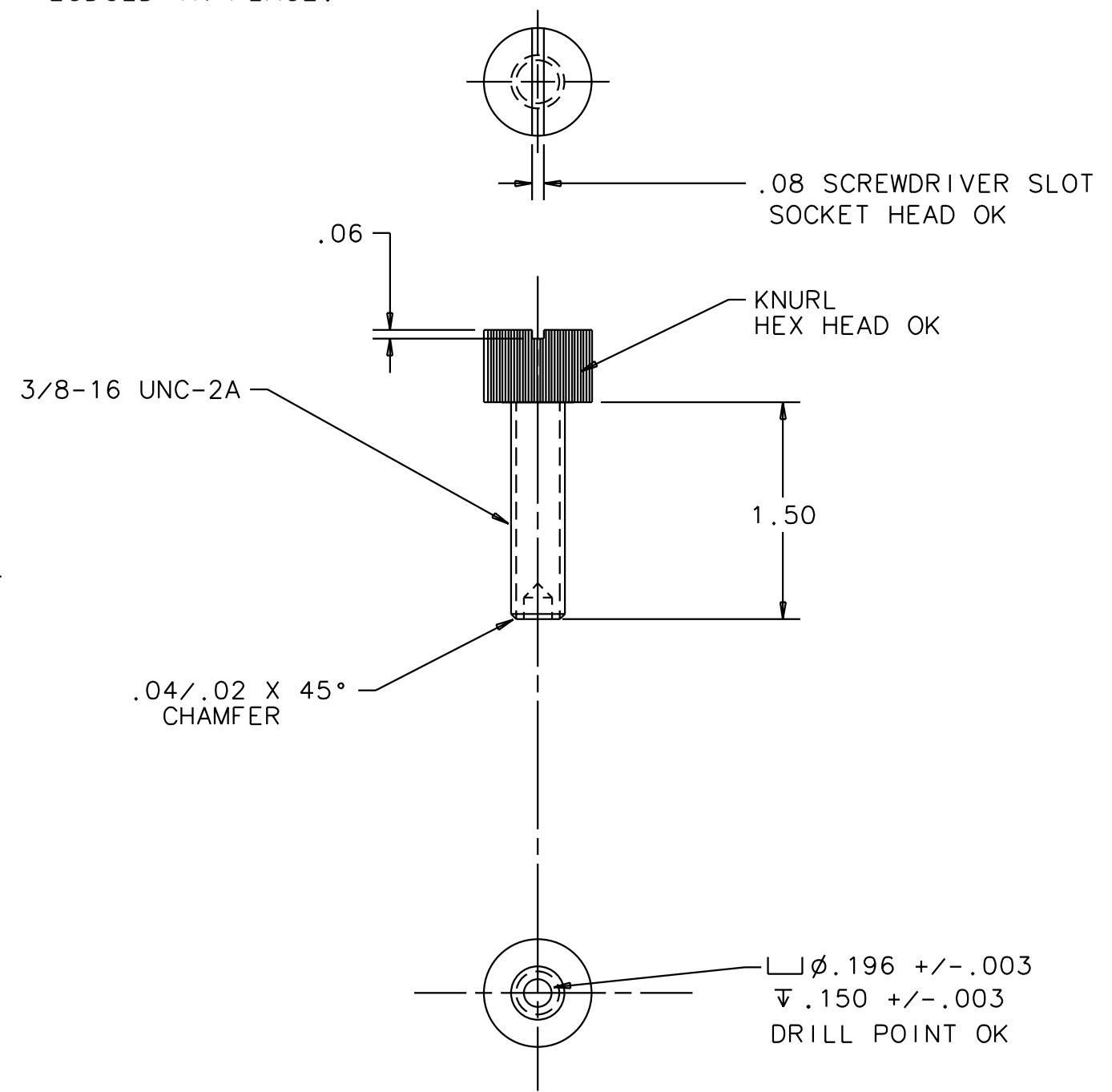
SCREW DETAIL ITEM 1
