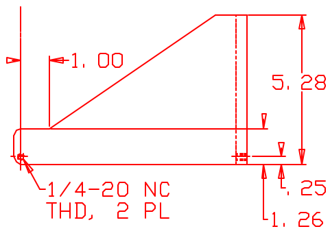
-1 SKIRT (RH & LH) MATERIAL: STAINLESS STEEL, TYPE 304, 304L, 316 OR 316L
