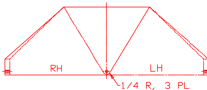
-1 SKIRT (RH & LH) MATERIAL: STAINLESS STEEL, TYPE 304, 304L, 316 OR 316L
