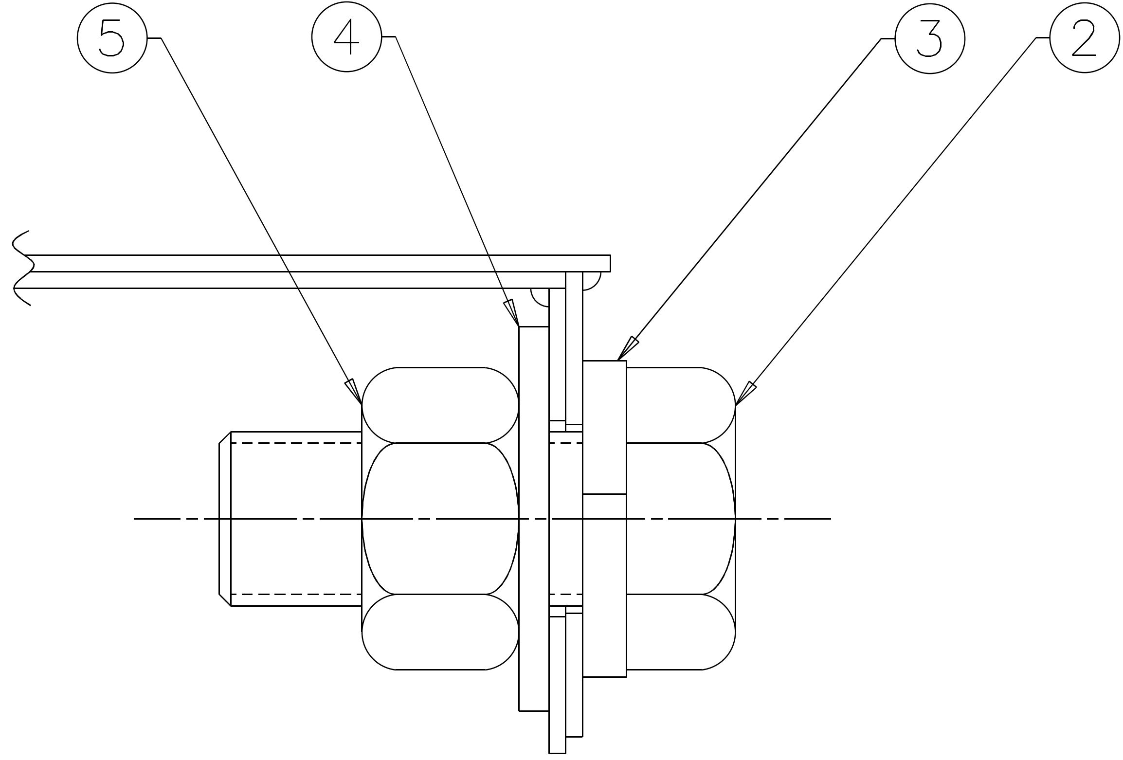
DETAIL D 4 FASTENING HARDWARE 2 PL 4
