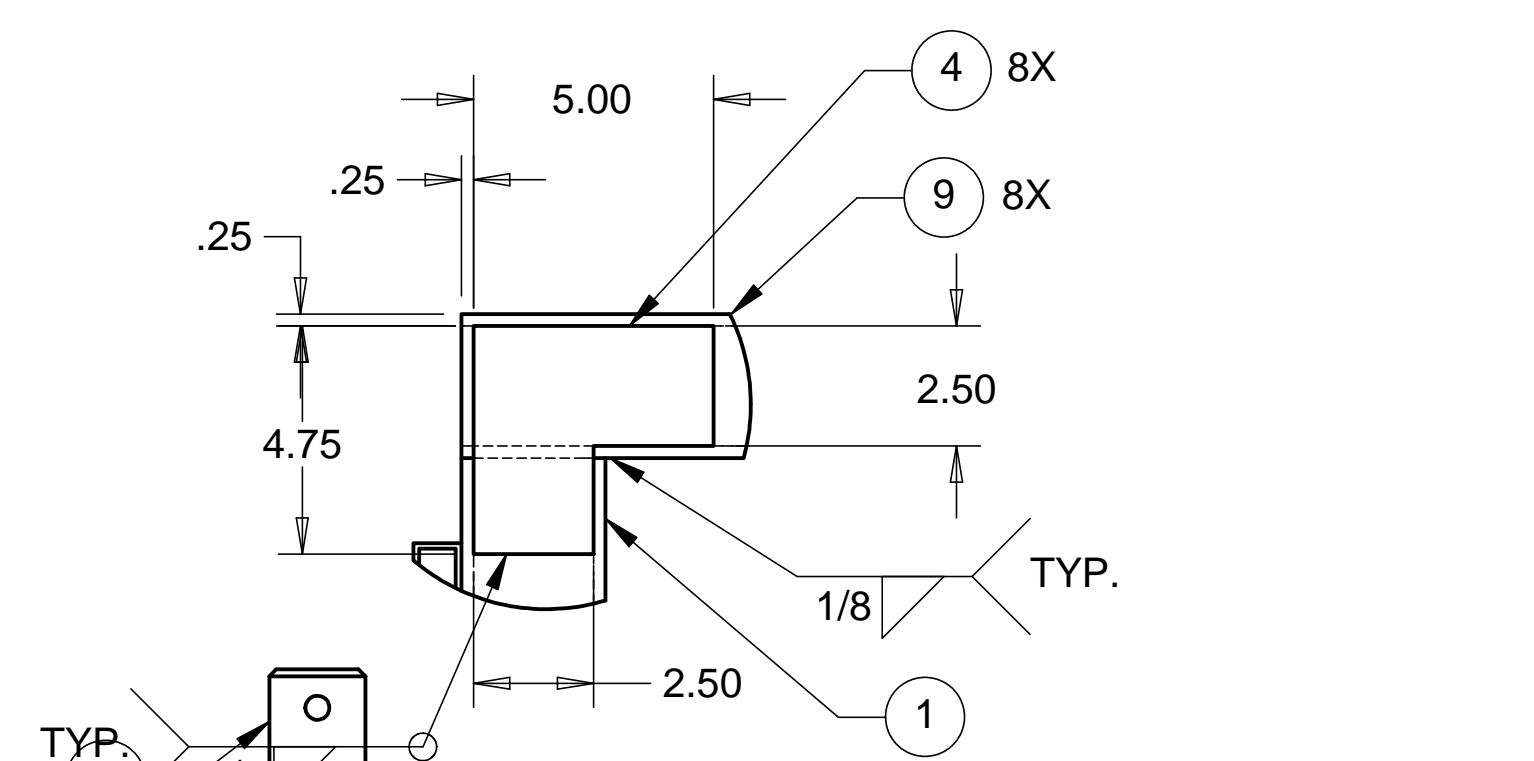
DETAIL B SCALE 1 : 4
